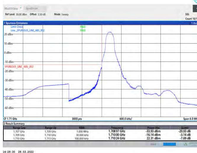
Band66-1.4MHz-QPSK-131979-6RB#0
