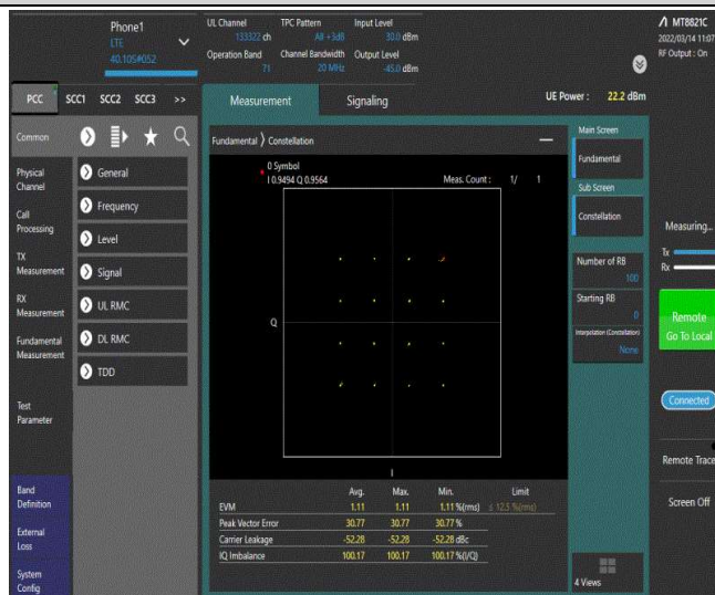
Band71-20MHz-16QAM-133322-100RB#0
