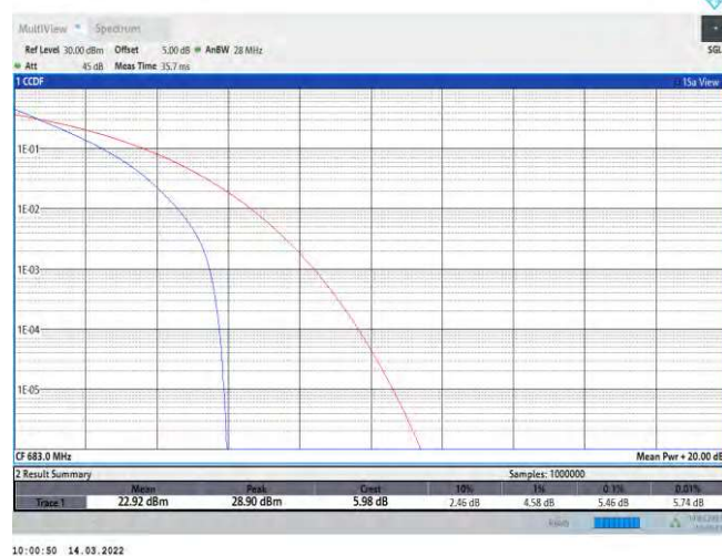
Band71-20MHz-QPSK-133322-100RB#0
