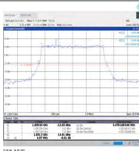
1-N2-15-5-L-2-DFT-PI2BPSK-Outer_Full-25@0-Ant1 -4.478-4.970-≤5-PASS
