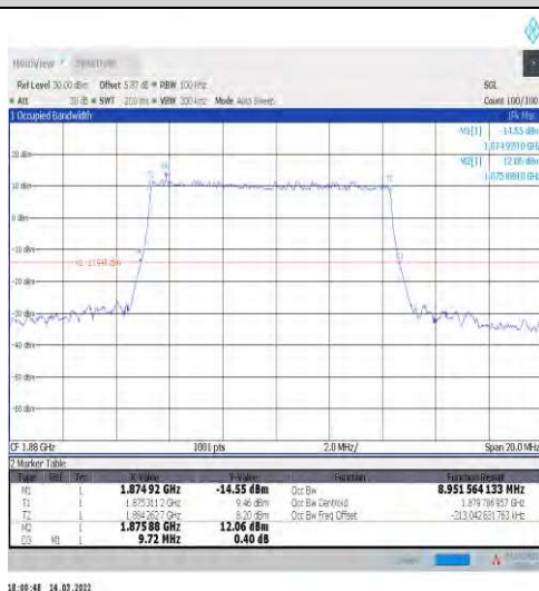
1-N2-15-10-M-3-DFT-16QAM-Outer_Full-50@0-Ant1-8.952-9.720-≤10-PASS
