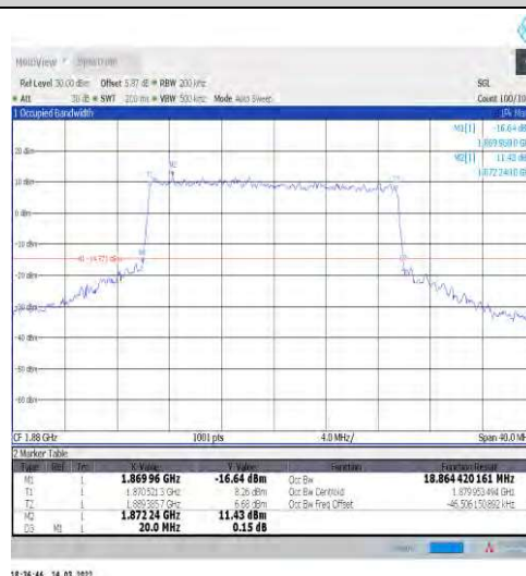
1-N2-15-20-M-6-CP-QPSK-Outer_Full-106@0-Ant 1-18.864-20.000-≤20-PASS
