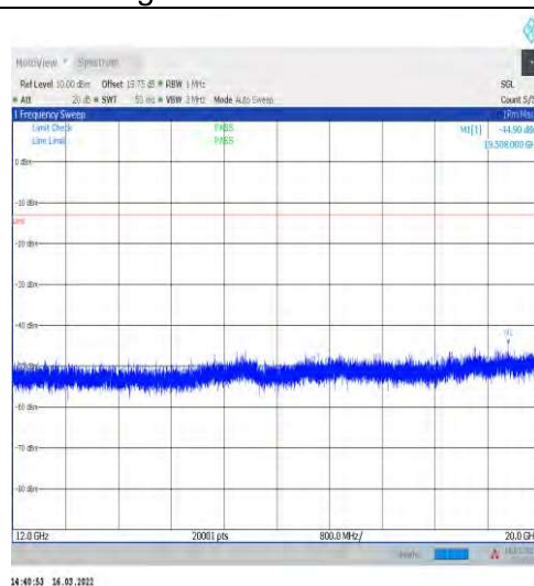
1-N2-15-20-L-1-DFT-PI2BPSK-Inner_1RB_Left-1@1 12000-20000-Ant1--44.90--13-PASS
