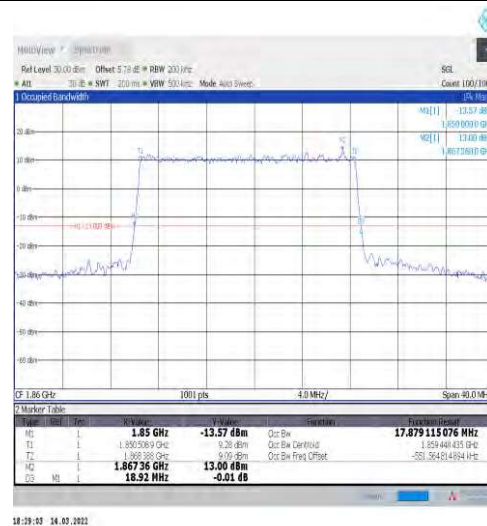
1-N2-15-20-L-3-DFT-16QAM-Outer_Full-100@0-Ant1 17.879-18.920≤20-PASS
