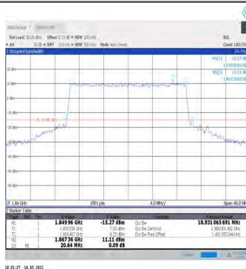
1-N2-15-20-L-7-CP-16QAM-Outer_Full-106@0-Ant1 18.931-20.640-≤20-PASS
