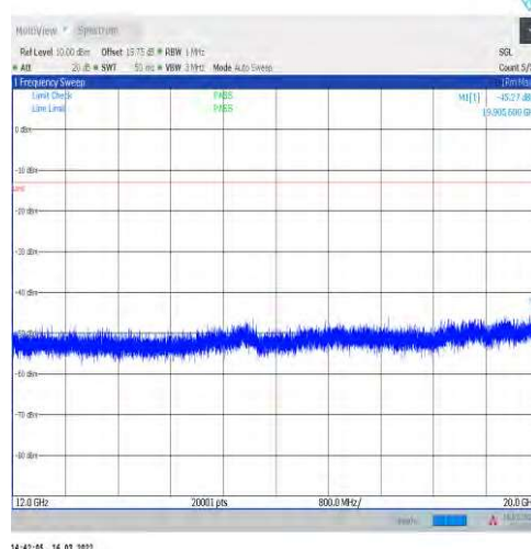
1-N2-15-20-M-1-DFT-PI2BPSK-Inner_1RB_Left-1@1 -12000-20000-Ant1--45.27--13-PASS
