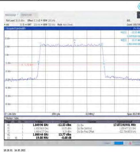
1-N2-15-20-L-1-DFT-QPSK-Outer_Full-100@0-Ant1 17.873-19.080≤20-PASS
