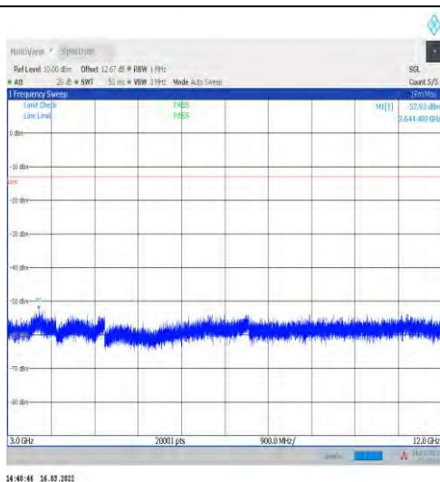
1-N2-15-20-L-1-DFT-PI2BPSK-Inner_1RB_Left-1@1 -3000-12000-Ant1--52.93--13-PASS
