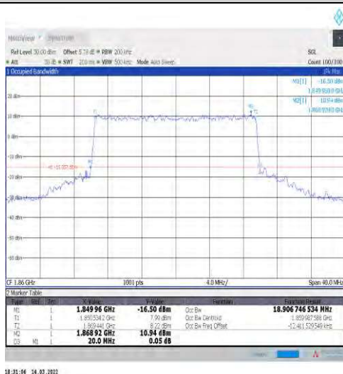
1-N2-15-20-L-6-CP-QPSK-Outer_Full-106@0-Ant1 18.907-20.000-≤20-PASS
