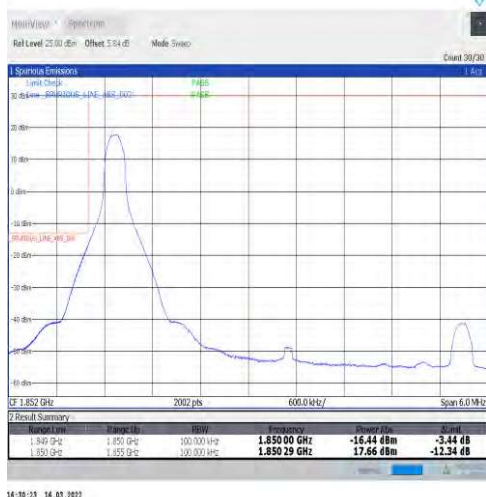
1-N2-15-5-L-4-CP-QPSK-Edge_1RB_Left-1@0-Ant1-seegraph-PASS-see graph
