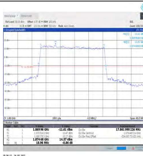
1-N2-15-20-M-2-DFT-PI2BPSK-Outer_Full-100@0-Ant1 1-17.862-18.960-≤20-PASS
