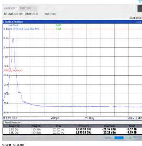
1-N2-15-20-L-4-CP-QPSK-Edge_1RB_Left-1@0-Ant1-seegraph-PASS-see graph
