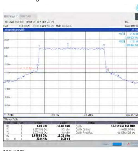
1-N2-15-20-H-7-CP-16QAM-Outer_Full-106@0-Ant1 -18.919-20.000-≤20-PASS
