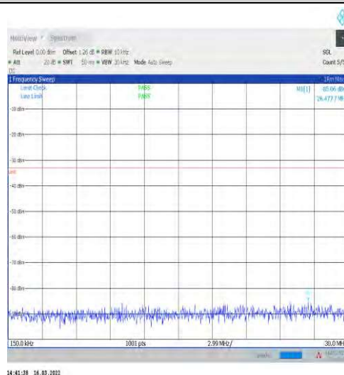
1-N2-15-20-M-1-DFT-PI2BPSK-Inner_1RB_Left-1@1 -0.15-30-Ant1--85.06--33-PASS
