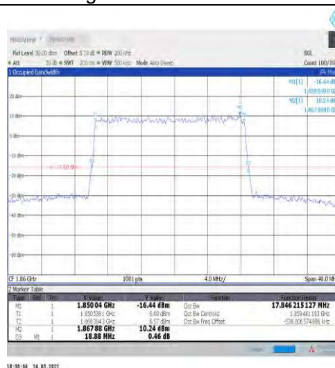
1-N2-15-20-L-5-DFT-256QAM-Outer_Full-100@0-Ant 1-17.846-18.880-≤20-PASS
