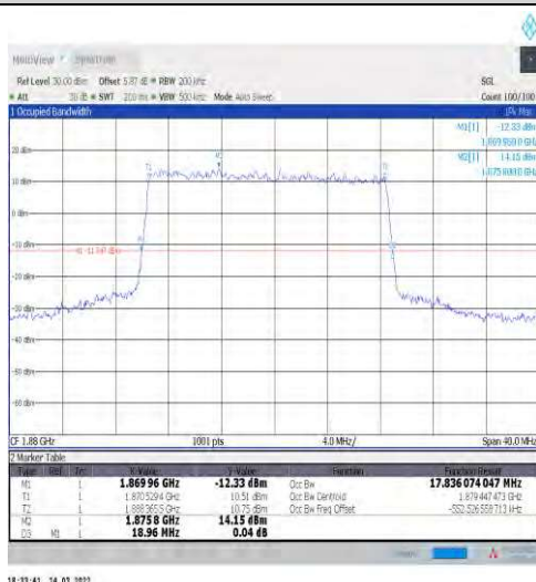
1-N2-15-20-M-1-DFT-QPSK-Outer_Full-100@0-Ant1 -17.836-18.960-≤20-PASS
