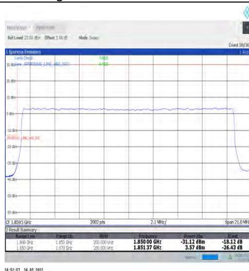
1-N2-15-20-L-3-DFT-PI2BPSK-Outer_Full-100@0-Ant1-seegraph-PASS-see graph
