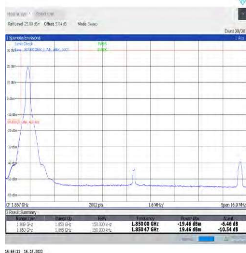
1-N2-15-15-L-4-CP-QPSK-Edge_1RB_Left-1@0-Ant1-seegraph-PASS-see graph
