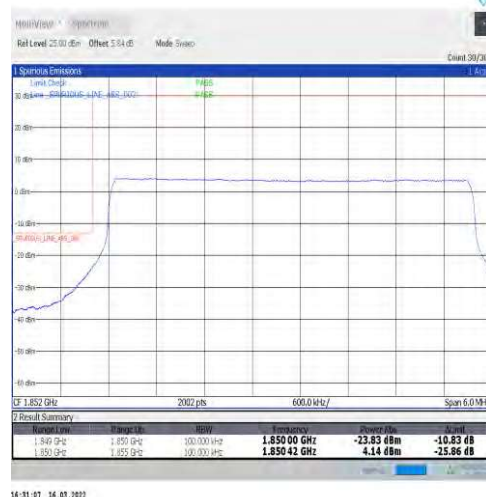
1-N2-15-5-L-6-CP-QPSK-Outer_Full-25@0-Ant1-seegraph-PASS-see graph
