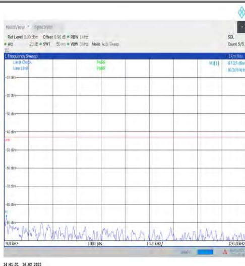
1-N2-15-20-M-1-DFT-PI2BPSK-Inner_1RB_Left-1@1 1-0.009-0.15-Ant1--87.35--43-PASS
