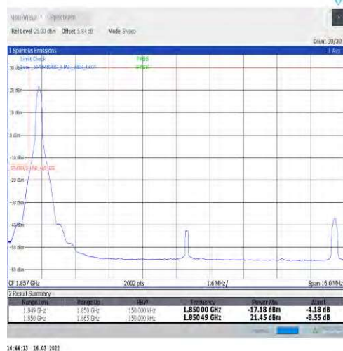
1-N2-15-15-L-1-DFT-PI2BPSK-Edge_1RB_Left-1@0-Ant1-seegraph-PASS-see graph
