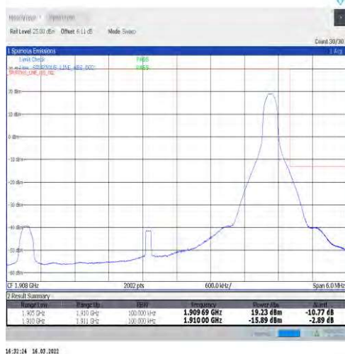
1-N2-15-5-H-2-DFT-PI2BPSK-Edge_1RB_Right-1@24-Ant1-seegraph-PASS-see graph
