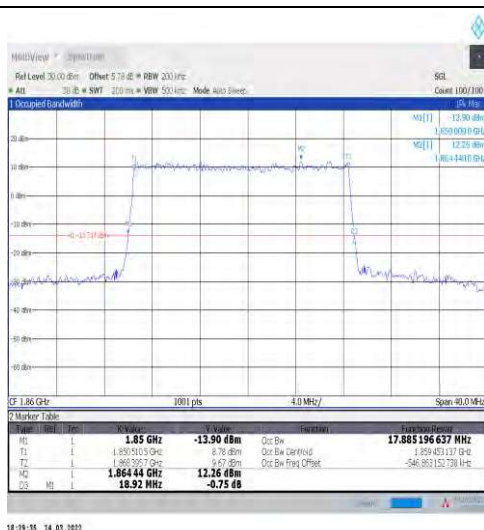
1-N2-15-20-L-4-DFT-64QAM-Outer_Full-100@0-Ant 1-17.885-18.920-≤20-PASS
