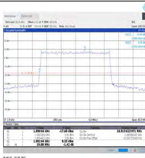
1-N2-15-20-H-9-CP-256QAM-Outer_Full-106@0-Ant1 1-18.916-19.880-≤20-PASS
