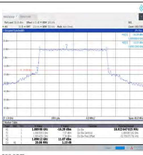
1-N2-15-20-H-6-CP-QPSK-Outer_Full-106@0-Ant1- 18.924-20.080-≤20-PASS
