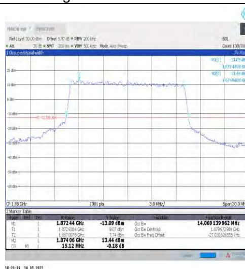
1-N2-15-15-M-7-CP-16QAM-Outer_Full-79@0-Ant1-1 14.069-15.120≤15-PASS
