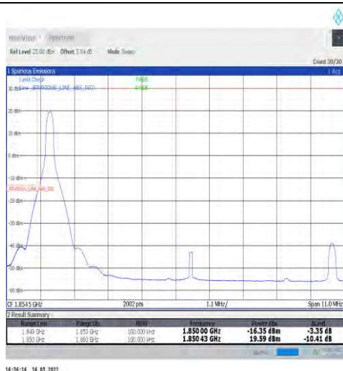
1-N2-15-10-L-1-DFT-PI2BPSK-Edge_1RB_Left-1@0-Ant1-seegraph-PASS-see graph
