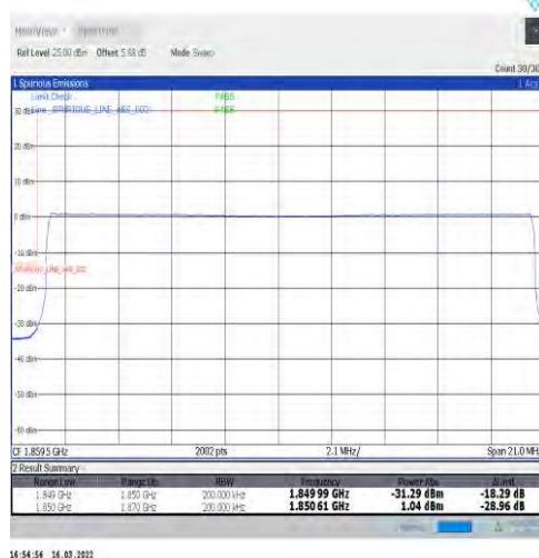
1-N2-15-20-L-6-CP-QPSK-Outer_Full-106@0-Ant1-seegraph-PASS-see graph
