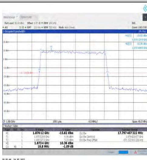
1-N2-15-20-M-5-DFT-256QAM-Outer_Full-100@0-Ant 1-17.797-18.800-≤20-PASS
