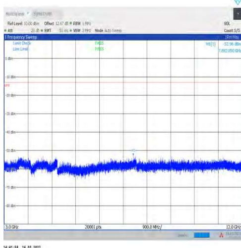
1-N2-15-20-M-1-DFT-PI2BPSK-Inner_1RB_Left-1@ 1-3000-12000-Ant1--52.96--13-PASS
