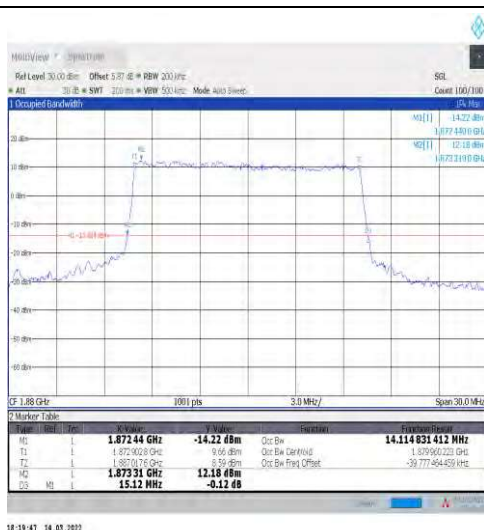
1-N2-15-15-M-6-CP-QPSK-Outer_Full-79@0-Ant1-1 4.115-15.120≤15-PASS
