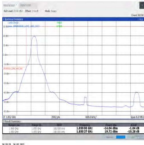
1-N2-15-5-L-1-DFT-PI2BPSK-Edge_1RB_Left-1@0-Ant1-seegraph-PASS-see graph
