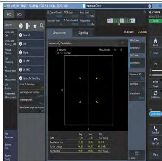
1-N41-30-100-M-2-DFT-QPSK-Outer_Full-270@0-Ant1-see graph-PASS
