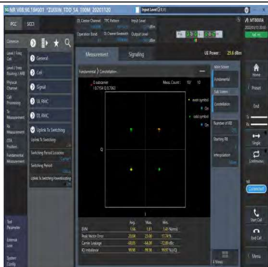
1-N41-30-100-M-1-DFT-PI2BPSK-Outer_Full-270@0-Ant1-see graph-PASS
