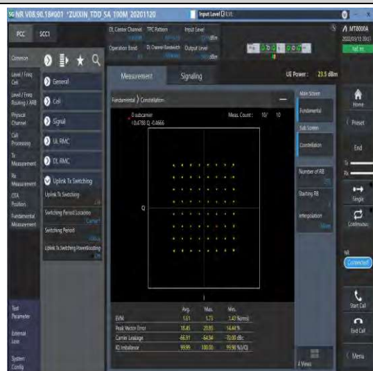
1-N41-30-100-M-4-DFT-64QAM-Outer_Full-270@0-Ant1-see graph-PASS
