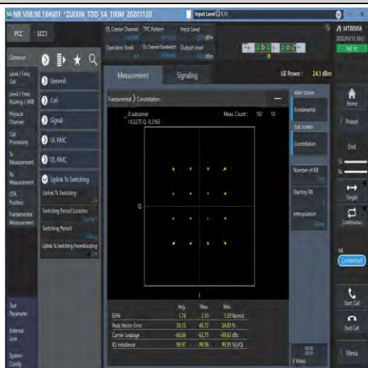
1-N41-30-100-M-3-DFT-16QAM-Outer_Full-270@0-Ant1-see graph-PASS
