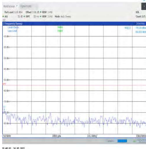
1-N41-30-100-H-1-DFT-PI2BPSK-Inner_1RB_Left-1 @1-0.009-0.15-Ant1--78.10--55-PASS
