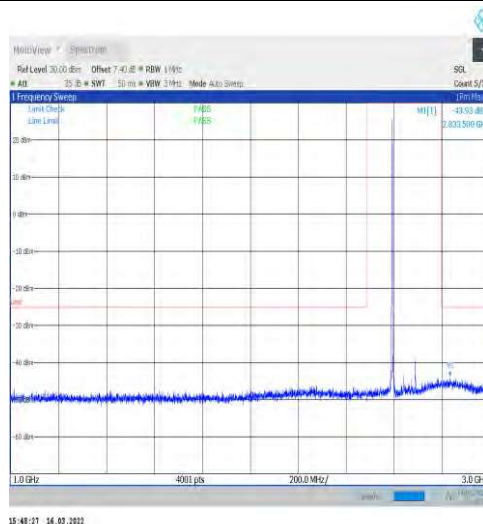
1-N41-30-100-H-1-DFT-PI2BPSK-Inner_1RB_Left-1 @1-1000-3000-Ant1--43.93--25-PASS
