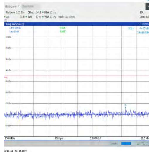
1-N41-30-100-M-1-DFT-PI2BPSK-Inner_1RB_Left-1 @1-0.15-30-Ant1--74.72--45-PASS
