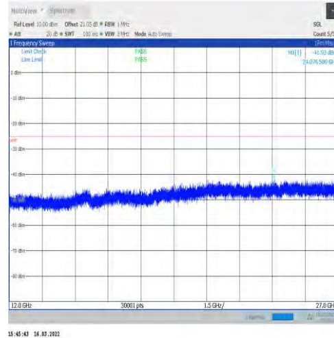
1-N41-30-100-L-1-DFT-PI2BPSK-Inner_1RB_Left-1 @1-12000-27000-Ant1--41.93--25-PASS
