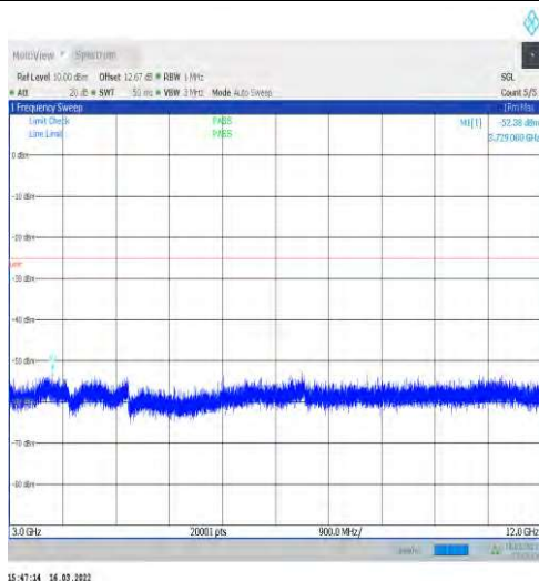
1-N41-30-100-M-1-DFT-PI2BPSK-Inner_1RB_Left-1 @1-3000-12000-Ant1--52.38--25-PASS
