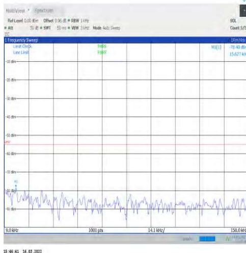
1-N41-30-100-M-1-DFT-PI2BPSK-Inner_1RB_Left-1 @1-0.009-0.15-Ant1--78.40--55-PASS
