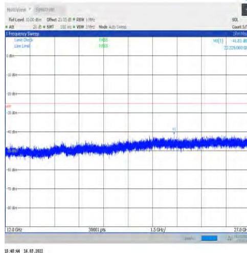
1-N41-30-100-H-1-DFT-PI2BPSK-Inner_1RB_Left-1 @1-12000-27000-Ant1--41.81--25-PASS
