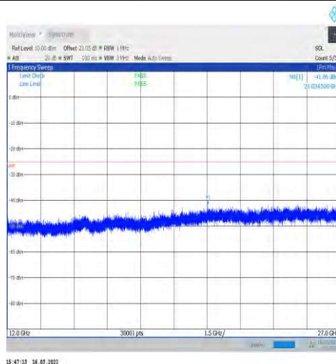
1-N41-30-100-M-1-DFT-PI2BPSK-Inner_1RB_Left-1 @1-12000-27000-Ant1--41.86--25-PASS
