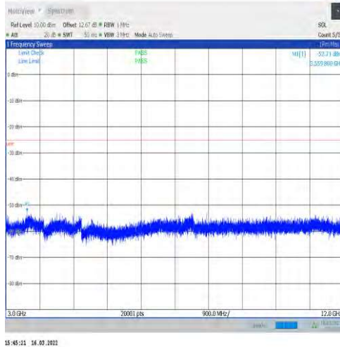
1-N41-30-100-L-1-DFT-PI2BPSK-Inner_1RB_Left-1 @1-3000-12000-Ant1--52.71--25-PASS
