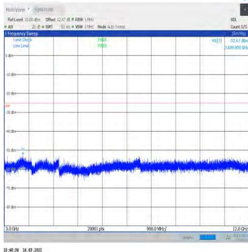
1-N41-30-100-H-1-DFT-PI2BPSK-Inner_1RB_Left-1 @1-3000-12000-Ant1--52.67--25-PASS
