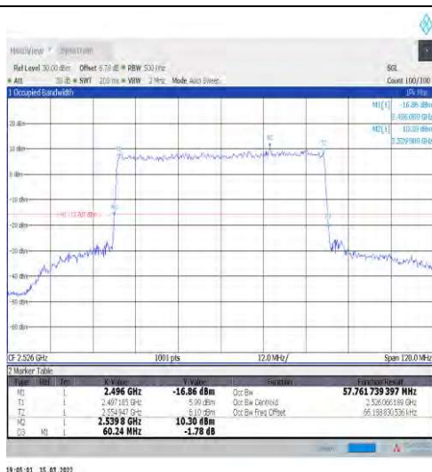
1-N41-30-60-L-9-CP-256QAM-Outer_Full-162@0-An t1-57.762-60.240-≤60-PASS
