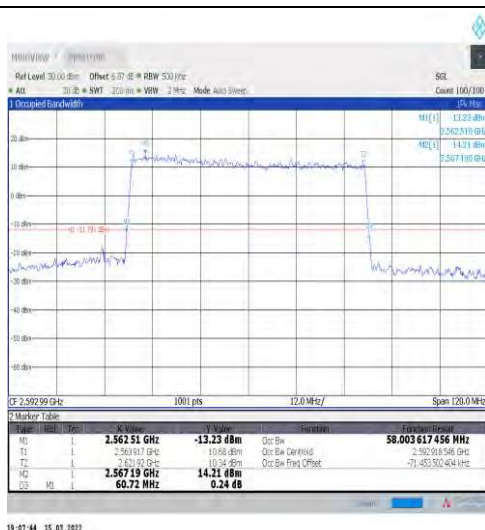
1-N41-30-60-M-4-DFT-64QAM-Outer_Full-162@0-A nt1-58.004-60.720-≤60-PASS
