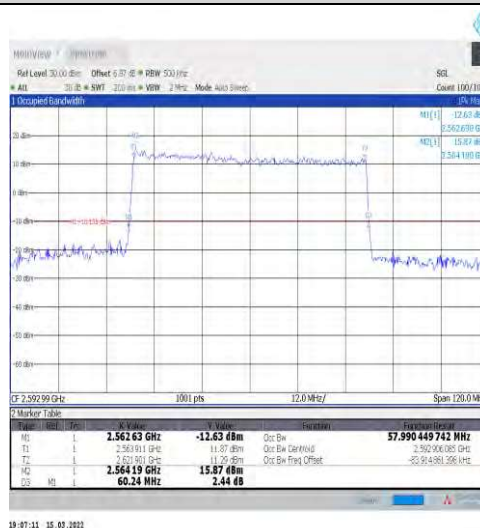
1-N41-30-60-M-3-DFT-16QAM-Outer_Full-162@0-A nt1-57.99-60.240-≤60-PASS
