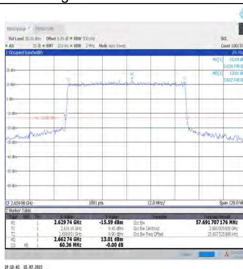
1-N41-30-60-H-8-CP-64QAM-Outer_Full-162@0-Ant 1-57.692-60.360-≤60-PASS
