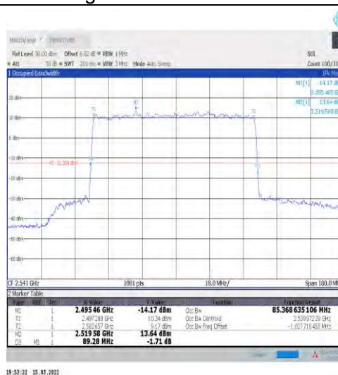
1-N41-30-90-L-5-DFT-256QAM-Outer_Full-240@0-A nt1-85.369-89.280-≤90-PASS
