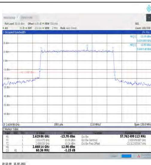
1-N41-30-60-H-7-CP-16QAM-Outer_Full-162@0-Ant 1-57.762-60.360-≤60-PASS
