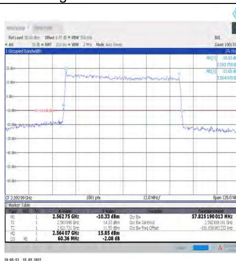
1-N41-30-60-M-1-DFT-QPSK-Outer_Full-162@0-Ant 1-57.825-60.360-≤60-PASS
