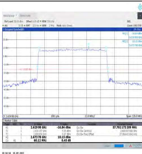
1-N41-30-60-H-9-CP-256QAM-Outer_Full-162@0-A nt1-57.702-60.120-≤60-PASS
