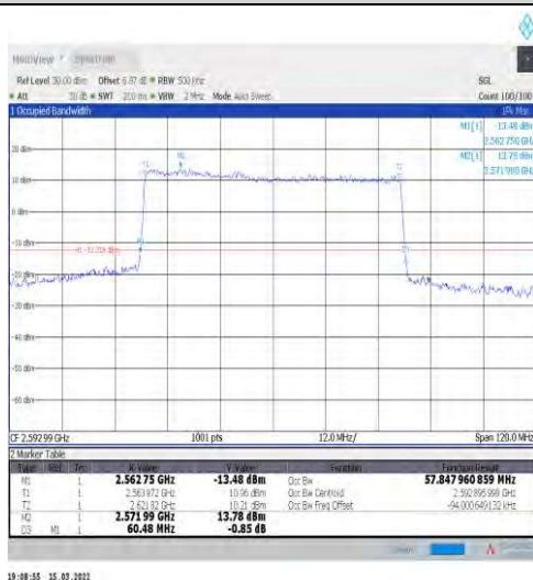
1-N41-30-60-M-6-CP-QPSK-Outer_Full-162@0-Ant1 -57.848-60.480-≤60-PASS
