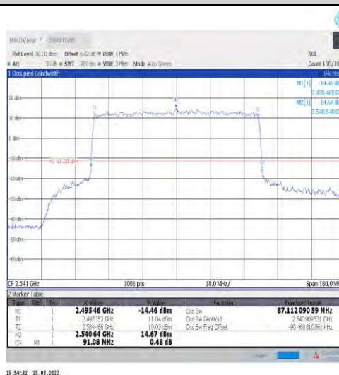
1-N41-30-90-L-7-CP-16QAM-Outer_Full-245@0-Ant 1-87.112-91.080-≤90-PASS
