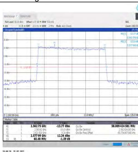
1-N41-30-60-M-5-DFT-256QAM-Outer_Full-162@0-A Ant1-58.009-60.480-≤60-PASS
