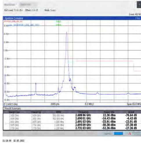
1-N41-30-40-H-2-DFT-PI2BPSK-Edge_1RB_Right-1@105-Ant1-PASS-see graph
