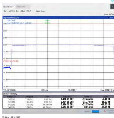
1-N41-30-100-L-6-CP-QPSK-Outer_Full-273@0-Ant1-PASS-see graph
