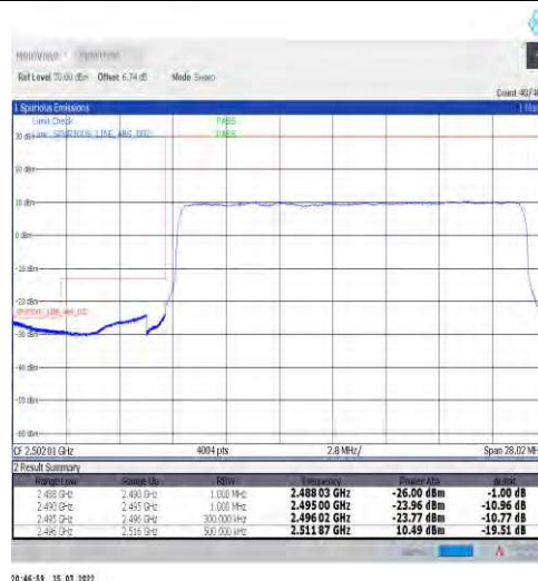
1-N41-30-20-L-3-DFT-PI2BPSK-Outer_Full-50@0-Ant1-PASS-see graph
