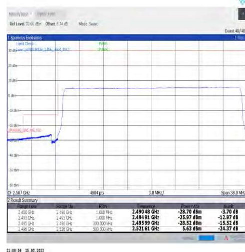
1-N41-30-30-L-6-CP-QPSK-Outer_Full-78@0-Ant1-PASS-see graph
