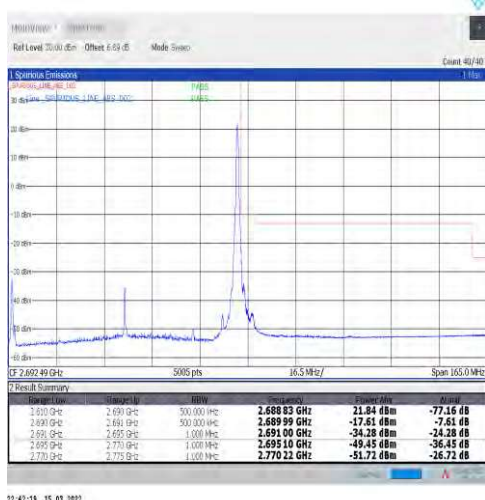
1-N41-30-80-H-5-CP-QPSK-Edge_1RB_Right-1@216- Ant1-PASS-see graph
