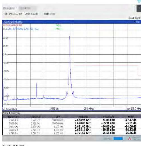
1-N41-30-100-H-5-CP-QPSK-Edge_1RB_Right-1@272 -Ant1-PASS-see graph
