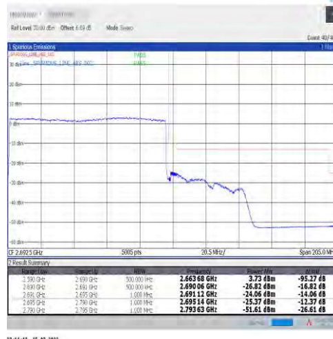
1-N41-30-100-H-3-DFT-PI2BPSK-Outer_Full-270 @0-Ant1-PASS-see graph
