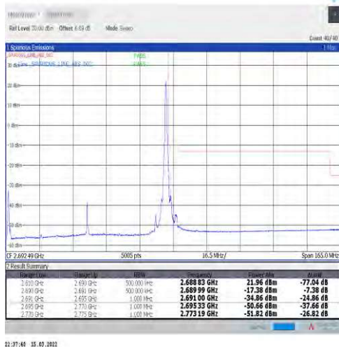
1-N41-30-80-H-2-DFT-PI2BPSK-Edge_1RB_Right-1@ 216-Ant1-PASS-see graph
