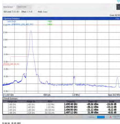
1-N41-30-30-L-4-CP-QPSK-Edge_1RB_Left-1@0-Ant1-PASS-see graph
