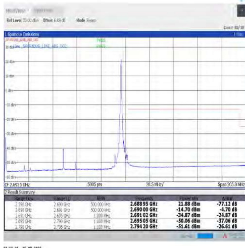
1-N41-30-100-H-2-DFT-PI2BPSK-Edge_1RB_Right-1 @272-Ant1-PASS-see graph
