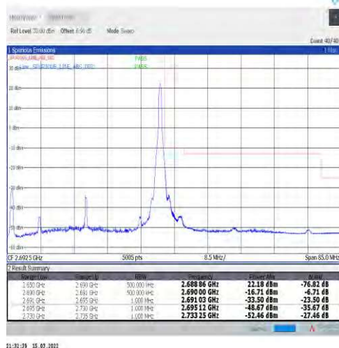
1-N41-30-40-H-5-CP-QPSK-Edge_1RB_Right-1@105-Ant1-PASS-see graph
