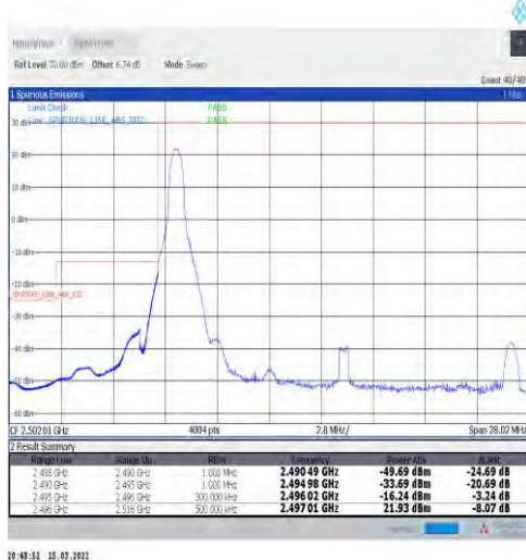
1-N41-30-20-L-4-CP-QPSK-Edge_1RB_Left-1@0-Ant1-PASS-see graph
