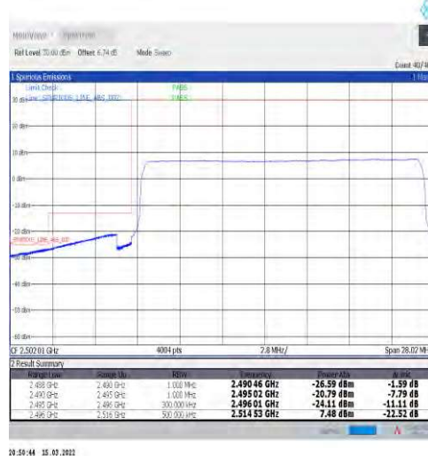
1-N41-30-20-L-6-CP-QPSK-Outer_Full-51@0-Ant1-PASS-see graph
