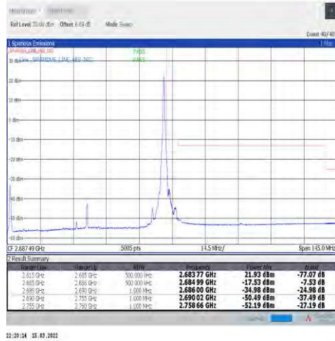
1-N41-30-70-H-2-DFT-PI2BPSK-Edge_1RB_Right-1@188-Ant1-PASS-see graph
