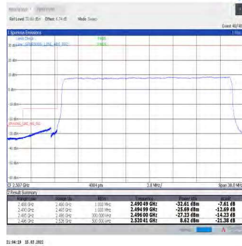
1-N41-30-30-L-3-DFT-PI2BPSK-Outer_Full-75@0-Ant1-PASS-see graph
