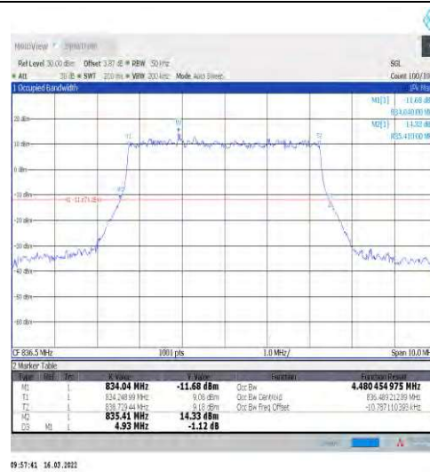
1-N5-15-5-M-1-DFT-QPSK-Outer_Full-25@0-Ant1-4.48-4.930-≤5-PASS
