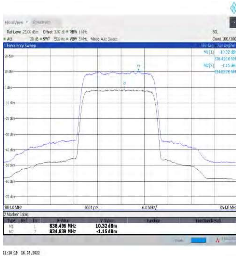
1-N5-15-20-L-1-DFT-256QAM-Outer_Full-100@0-Ant t1-11.47-100%-0.00-11.47-PASS-≤13
