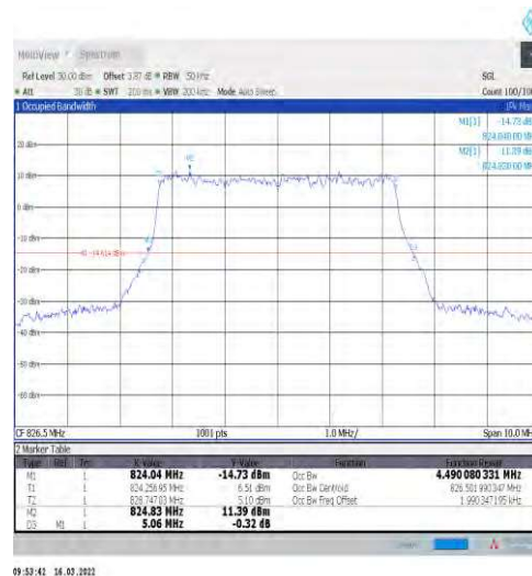
1-N5-15-5-L-4-DFT-64QAM-Outet_Full-25@0-Ant1-4 .49-5.060-≤5-PASS
