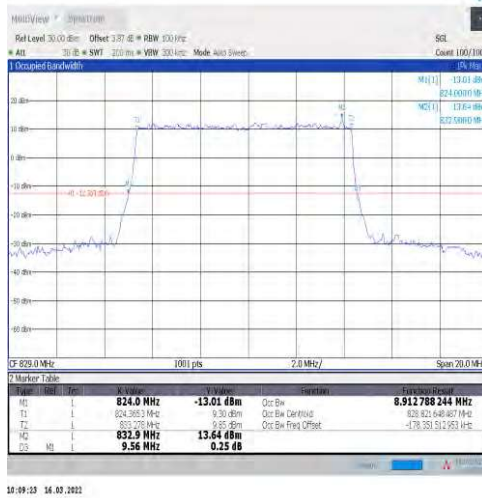
1-N5-15-10-L-2-DFT-PI2BPSK-Outer_Full-50@0-Ant 1-8.913-9.560-≤10-PASS
