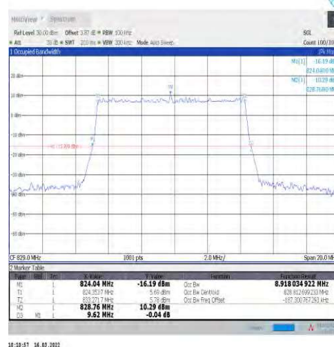
1-N5-15-10-L-5-DFT-256QAM-Outer_Full-50@0-Ant 1-8.918-9.620-≤10-PASS
