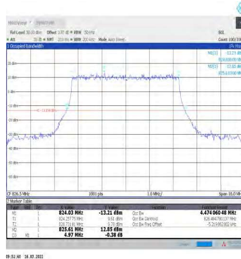
1-N5-15-5-L-2-DFT-PI2BPSK-Outet_Full-25@0-Ant1 -4.474-4.970-≤5-PASS
