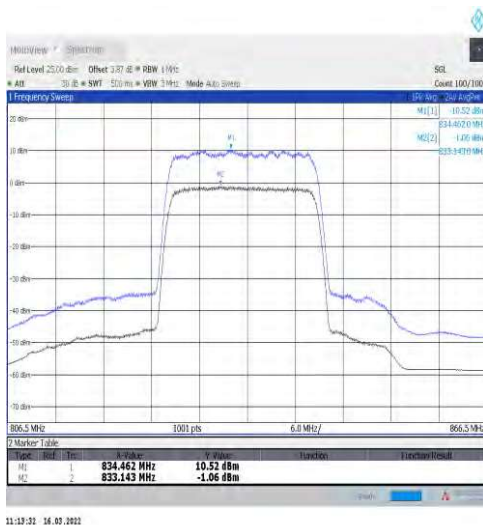
1-N5-15-20-M-1-DFT-256QAM-Outer_Full-100@0-A nt1-11.58-100%-0.00-11.58-PASS-≤13
