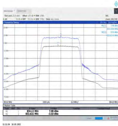
1-N5-15-20-L-2-CP-256QAM-Outer_Full-106@0-Ant t1-11.51-100%-0.00-11.51-PASS-≤13
