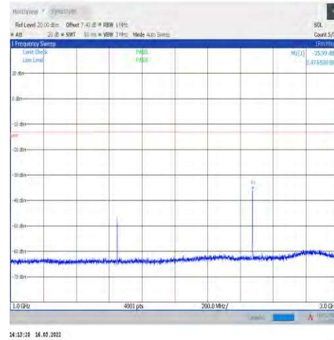
1-N5-15-20-L-1-DFT-PI2BPSK-Inner_1RB_Left-1@1 -1000-3000-Ant1--35.99--13-PASS
