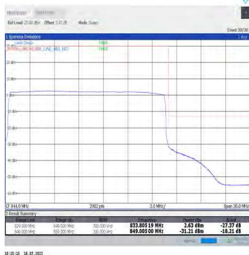
1-N5-15-20-H-6-CP-QPSK-Outer_Full-106@0-Ant1-seegraph-PASS-see graph
