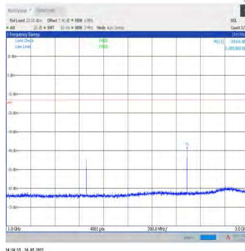
1-N5-15-20-H-1-DFT-PI2BPSK-Inner_1RB_Left-1@1 -1000-3000-Ant1--39.66--13-PASS
