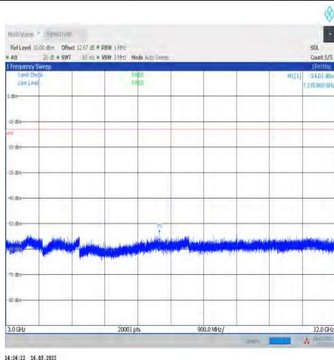
1-N5-15-20-H-1-DFT-PI2BPSK-Inner_1RB_Left-1@ 1-3000-12000-Ant1--54.01--13-PASS
