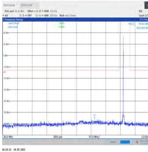
1-N5-15-20-L-1-DFT-PI2BPSK-Inner_1RB_Left-1@1 -30-1000-Ant1--55.66--13-PASS
