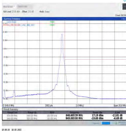
1-N5-15-10-H-5-CP-QPSK-Edge_1RB_Right-1@51-Ant1-seegraph-PASS-see graph
