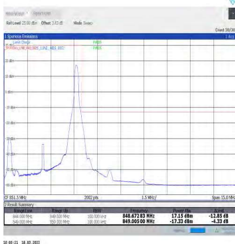
1-N5-15-5-H-5-CP-QPSK-Edge_1RB_Right-1@24-Ant1-seegraph-PASS-see graph
