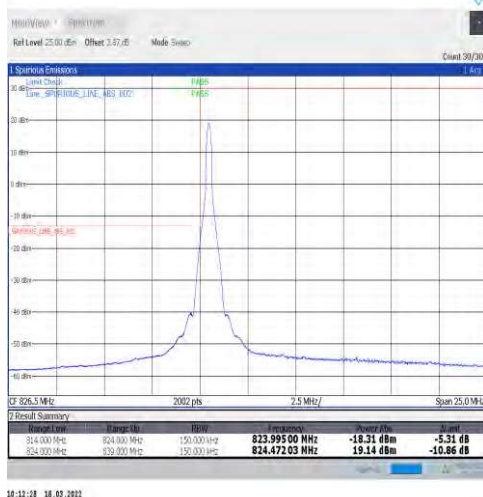
1-N5-15-15-L-4-CP-QPSK-Edge_1RB_Left-1@0-Ant1- seegraph-PASS-see graph
