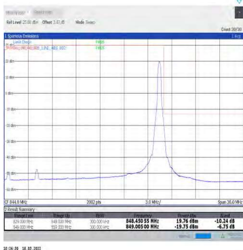
1-N5-15-20-H-5-CP-QPSK-Edge_1RB_Right-1@105-Ant1-seegraph-PASS-see graph
