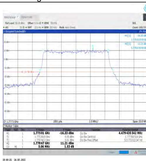
1-N66-15-5-H-4-DFT-64QAM-Outer_Full-25@0-Ant1 -4.479-5.060-≤5-PASS
