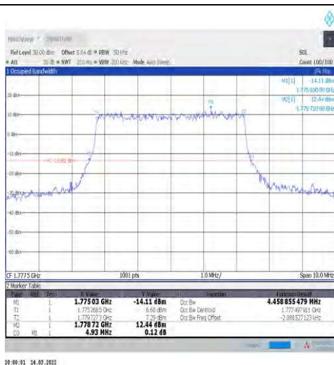
1-N66-15-5-H-3-DFT-16QAM-Outer_Full-25@0-Ant1 -4.459-4.930-≤5-PASS
