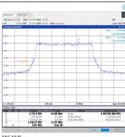
1-N66-15-5-M-4-DFT-64QAM-Outer_Full-25@0-Ant1 -4.484-5.070-≤5-PASS
