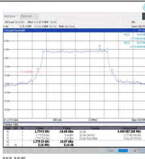
1-N66-15-5-H-6-CP-QPSK-Outer_Full-25@0-Ant1-4. 47-5.160-≤5-PASS
