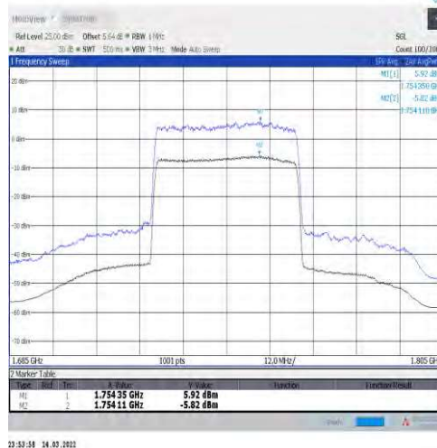
1-N66-15-40-M-2-CP-256QAM-Outer_Full-216@0-A nt1-11.74-100%-0.00-11.74-PASS-≤13
