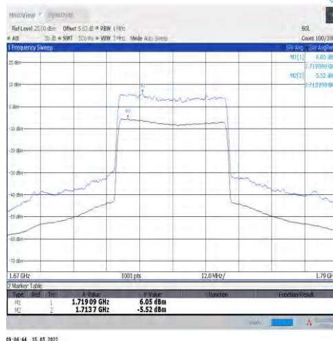
1-N66-15-40-L-2-CP-256QAM-Outer_Full-216@0-A nt1-11.57-100%-0.00-11.57-PASS-≤13
