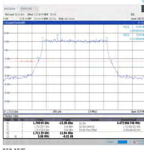
1-N66-15-5-L-2-DFT-PI2BPSK-Outer_Full-25@0-Ant1-4 1-4.474-5.080-≤5-PASS
