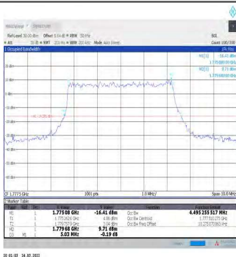
1-N66-15-5-H-5-DFT-256QAM-Outer_Full-25@0-Ant 1-4.495-5.030-≤5-PASS
