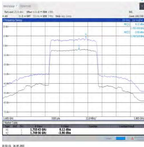
1-N66-15-40-M-1-DFT-256QAM-Outer_Full-216@0-A nt1-12.02-100%-0.00-12.02-PASS-≤13
