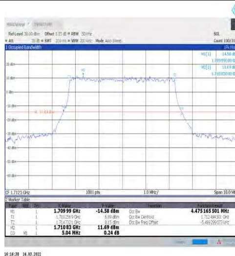
1-N66-15-5-L-4-DFT-64QAM-Outer_Full-25@0-Ant1-4 4.475-5.040-≤5-PASS
