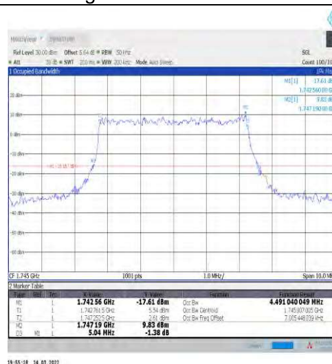
1-N66-15-5-M-5-DFT-256QAM-Outer_Full-25@0-Ant 1-4.491-5.040-≤5-PASS
