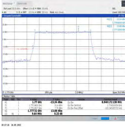
1-N66-15-10-H-4-DFT-64QAM-Outer_Full-50@0-Ant 1-8.94-9.640-≤10-PASS
