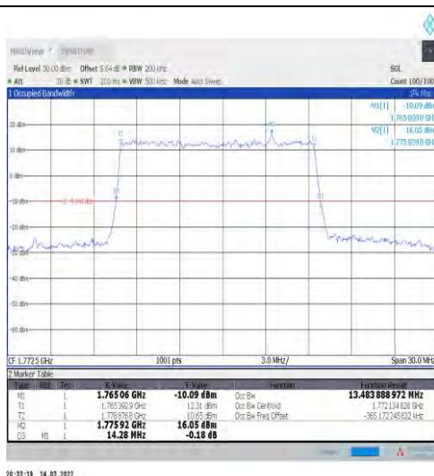
1-N66-15-15-H-1-DFT-QPSK-Outer_Full-75@0-Ant1 -13.484-14.280≤15-PASS
