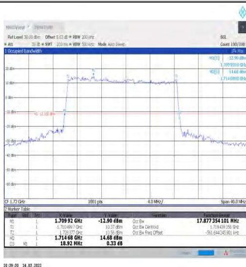
1-N66-15-20-L-2-DFT-PI2BPSK-Outer_Full-100@0-Ant 1-17.877-18.920-≤20-PASS
