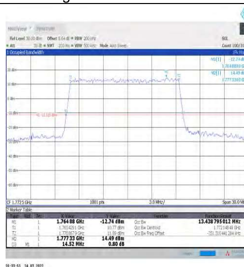
1-N66-15-15-H-2-DFT-PI2BPSK-Outer_Full-75@0-Ant1 -13.439-14.520≤15-PASS
