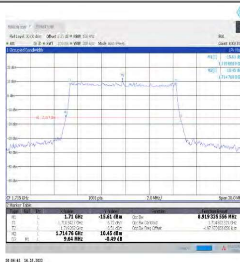
1-N66-15-10-L-5-DFT-256QAM-Outer_Full-50@0-Ant t1-8.919-9.640-≤10-PASS
