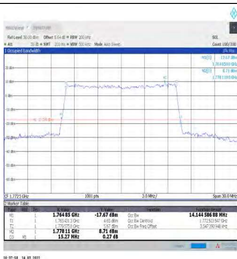
1-N66-15-15-H-9-CP-256QAM-Outer_Full-79@0-Ant 1-14.145-15.270-≤15-PASS
