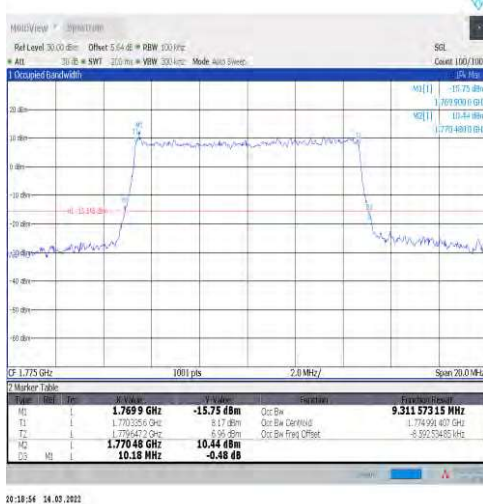
1-N66-15-10-H-6-CP-QPSK-Outer_Full-52@0-Ant1 9.312-10.180-≤10-PASS
