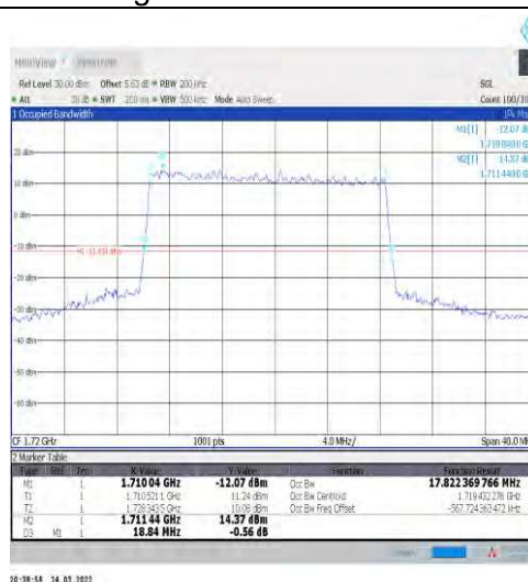
1-N66-15-20-L-1-DFT-QPSK-Outer_Full-100@0-Ant 1-17.822-18.840-≤20-PASS
