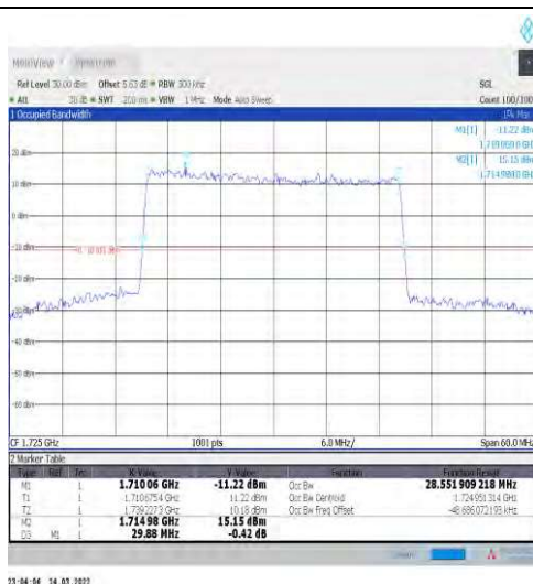
1-N66-15-30-L-1-DFT-QPSK-Outter_Full-160@0-Ant t1-28.552-29.880-≤30-PASS
