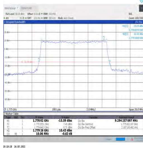
1-N66-15-10-H-7-CP-16QAM-Outer_Full-52@0-Ant1 -9.294-10.060-≤10-PASS
