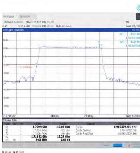
1-N66-15-10-L-2-DFT-PI2BPSK-Outer_Full-50@0-A nt1-8.915-9.680-≤10-PASS
