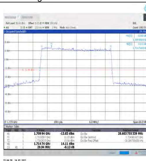
1-N66-15-30-L-2-DFT-PI2BPSK-Outter_Full-160@0-Ant t1-28.604-29.940-≤30-PASS
