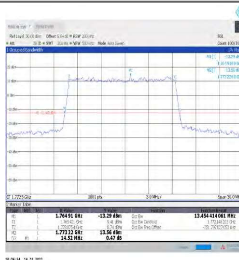
1-N66-15-15-H-4-DFT-64QAM-Outer_Full-75@0-Ant1 -1-13.454-14.520≤15-PASS
