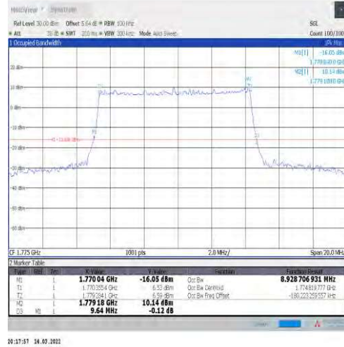
1-N66-15-10-H-5-DFT-256QAM-Outer_Full-50@0-Ant 1-8.929-9.640-≤10-PASS
