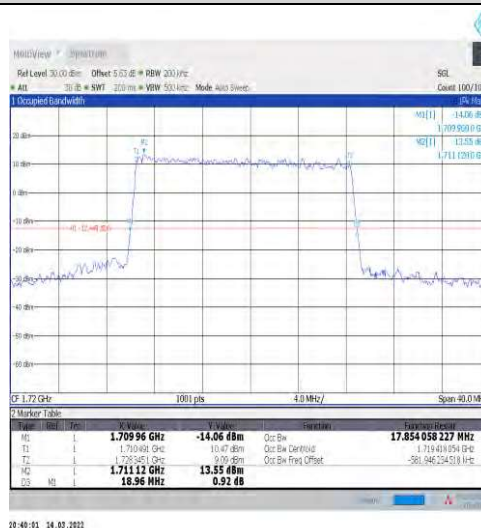
1-N66-15-20-L-3-DFT-16QAM-Outer_Full-100@0-Ant 1-17.854-18.960-≤20-PASS
