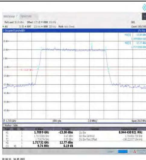
1-N66-15-10-L-4-DFT-64QAM-Outer_Full-50@0-Ant 1-8.944-9.740-≤10-PASS
