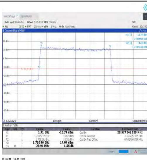
1-N66-15-30-L-3-DFT-16QAM-Outter_Full-160@0-Ant t1-28.577-29.940-≤30-PASS
