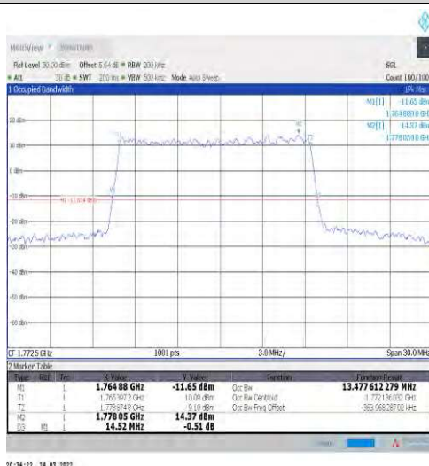
1-N66-15-15-H-3-DFT-16QAM-Outer_Full-75@0-Ant1 -1-13.478-14.520≤15-PASS
