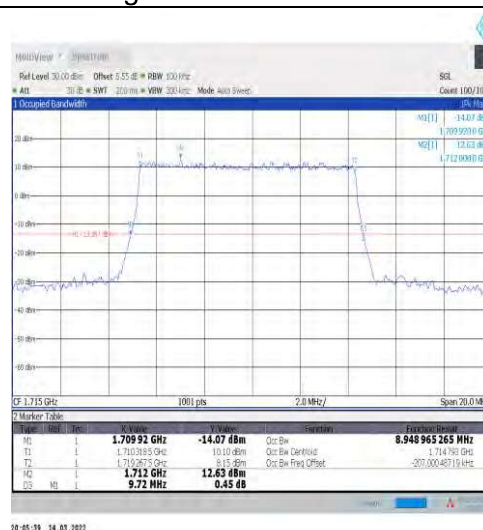
1-N66-15-10-L-3-DFT-16QAM-Outer_Full-50@0-Ant 1-8.949-9.720-≤10-PASS
