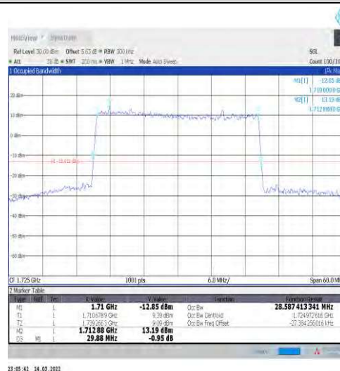
1-N66-15-30-L-4-DFT-64QAM-Outter_Full-160@0-Ant t1-28.587-29.880-≤30-PASS
