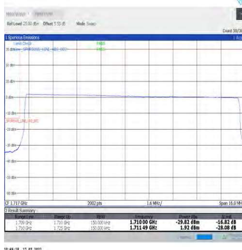
1-N66-15-15-L-6-CP-QPSK-Outer_Full-79@0-Ant1-seegraph-PASS-see graph
