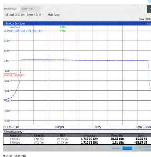
1-N66-15-10-L-6-CP-QPSK-Outer_Full-52@0-Ant1-seegraph-PASS-see graph
