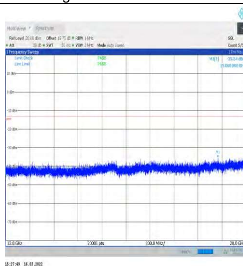
1-N66-15-40-L-1-DFT-PI2BPSK-Inner_1RB_Left-1@ 1-12000-20000-Ant1--35.54--13-PASS
