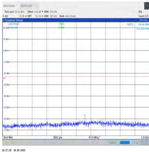
1-N66-15-40-L-1-DFT-PI2BPSK-Inner_1RB_Left-1@ 1-30-1000-Ant1--60.46--23-PASS
