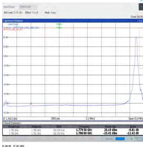
1-N66-15-30-H-5-CP-QPSK-Edge_1RB_Right-1@159-Ant1-seegraph-PASS-see graph
