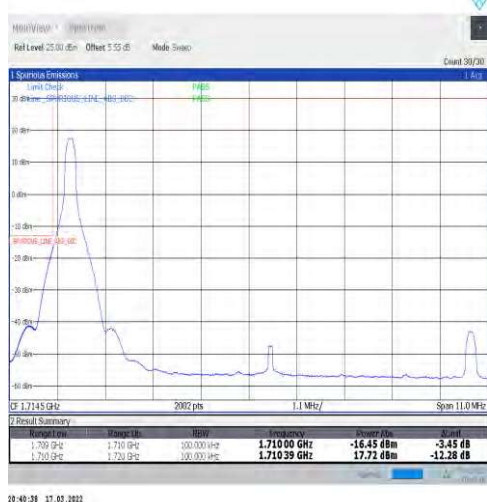
1-N66-15-10-L-4-CP-QPSK-Edge_1RB_Left-1@0-Ant1-seegraph-PASS-see graph
