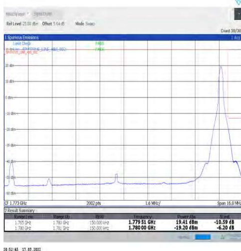
1-N66-15-15-H-5-CP-QPSK-Edge_1RB_Right-1@78-Ant1-seegraph-PASS-see graph
