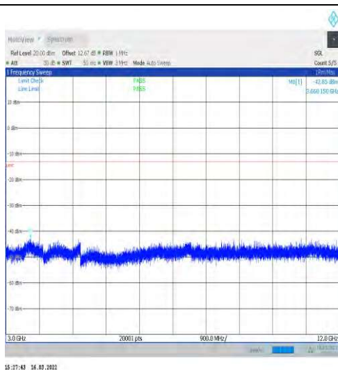
1-N66-15-40-L-1-DFT-PI2BPSK-Inner_1RB_Left-1@ 1-3000-12000-Ant1--42.85--13-PASS
