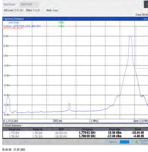
1-N66-15-10-H-2-DFT-PI2BPSK-Edge_1RB_Right-1@51-Ant1-seegraph-PASS-see graph
