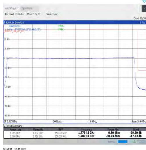
1-N66-15-15-H-6-CP-QPSK-Outer_Full-79@0-Ant1-seegraph-PASS-see graph
