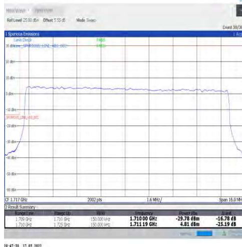
1-N66-15-15-L-3-DFT-PI2BPSK-Outer_Full-75@0-Ant1-seegraph-PASS-see graph
