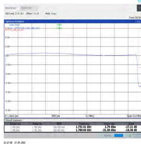
1-N66-15-40-H-6-CP-QPSK-Outer_Full-216@0-Ant1-seegraph-PASS-see graph
