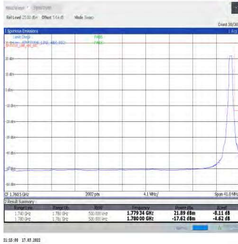
1-N66-15-40-H-2-DFT-PI2BPSK-Edge_1RB_Right-1@215-Ant1-seegraph-PASS-see graph
