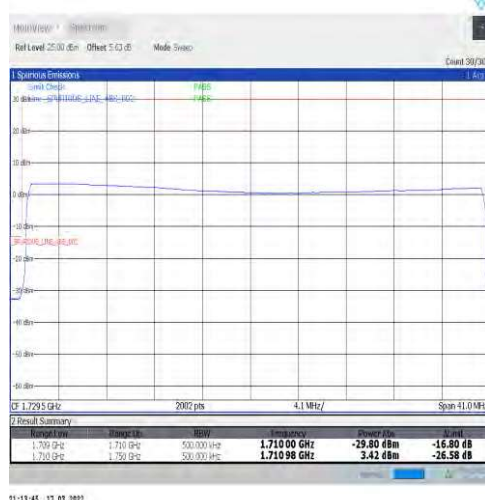
1-N66-15-40-L-6-CP-QPSK-Outer_Full-216@0-Ant1-seegraph-PASS-see graph
