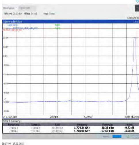
1-N66-15-40-H-5-CP-QPSK-Edge_1RB_Right-1@215-Ant1-seegraph-PASS-see graph
