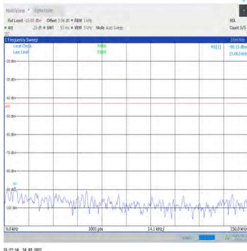
1-N66-15-40-L-1-DFT-PI2BPSK-Inner_1RB_Left-1@ 1-0.009-0.15-Ant1--90.15--43-PASS
