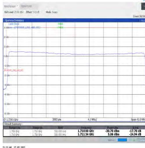
1-N66-15-40-L-3-DFT-PI2BPSK-Outer_Full-216@0-Ant1-seegraph-PASS-see graph
