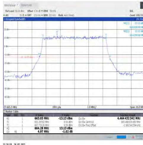
1-N71-15-5-L-2-DFT-PI2BPSK-Outer_Full-25@0-Ant1 1-4.464-4.970-≤5-PASS
