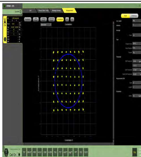
1-N71-15-20-M-4-DFT-64QAM-Outer_Full-100@0-A nt1-see graph-PASS
