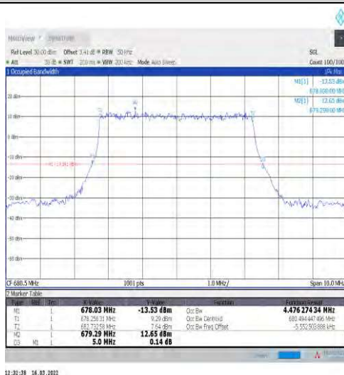
1-N71-15-5-M-2-DFT-PI2BPSK-Outer_Full-25@0-Ant1 t1-4.476-5.000-≤5-PASS
