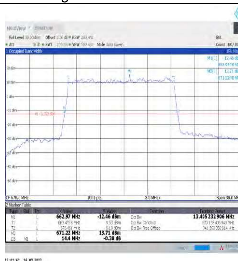
1-N71-15-15-L-4-DFT-64QAM-Outer_Full-75@0-Ant t1-13.405-14.400≤15-PASS
