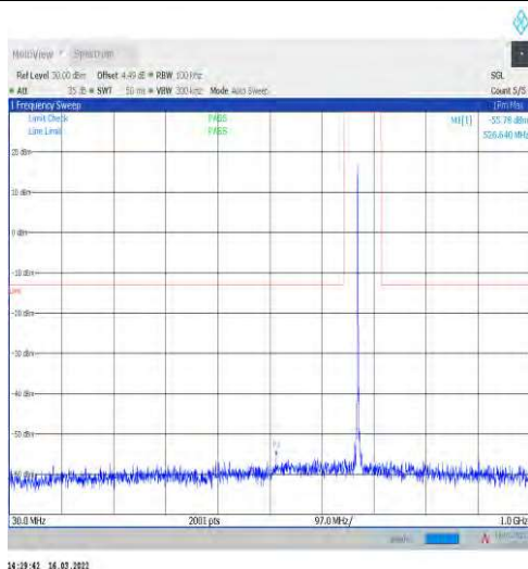
1-N71-15-20-H-1-DFT-PI2BPSK-Inner_1RB_Left-1 @1-30-1000-Ant1--55.78--13-PASS
