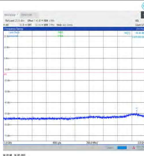
1-N71-15-20-H-1-DFT-PI2BPSK-Inner_1RB_Left-1@ 1-1000-3000-Ant1--48.46--13-PASS
