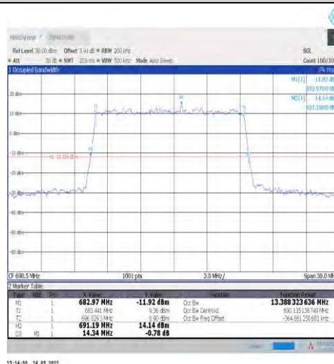
1-N71-15-15-H-4-DFT-64QAM-Outer_Full-75@0-Ant1 1-13.388-14.340≤15-PASS
