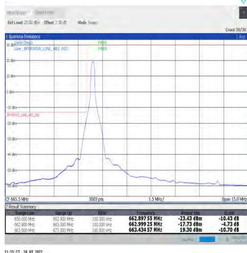
1-N71-15-10-L-1-DFT-PI2BPSK-Edge_1RB_Left-1@0-Ant1-PASS-see graph
