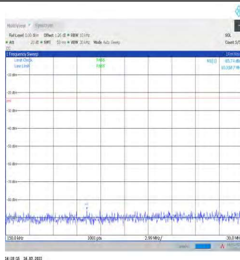
1-N71-15-20-M-1-DFT-PI2BPSK-Inner_1RB_Left-1@ 1-0.15-30-Ant1--85.74--23-PASS
