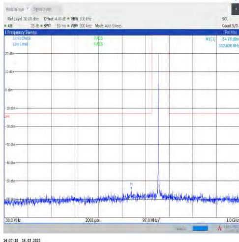
1-N71-15-20-L-1-DFT-PI2BPSK-Inner_1RB_Left-1@ 1-30-1000-Ant1--54.78--13-PASS
