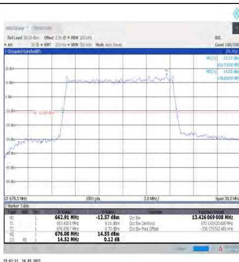
1-N71-15-15-L-3-DFT-16QAM-Outer_Full-75@0-Ant t1-13.426-14.520≤15-PASS
