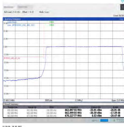
1-N71-15-10-L-6-CP-QPSK-Outer_Full-52@0-Ant1-PASS-see graph
