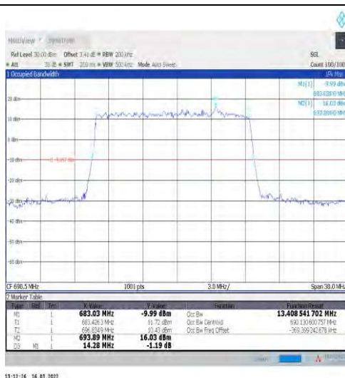
1-N71-15-15-H-1-DFT-QPSK-Outer_Full-75@0-Ant1 -13.409-14.280≤15-PASS
