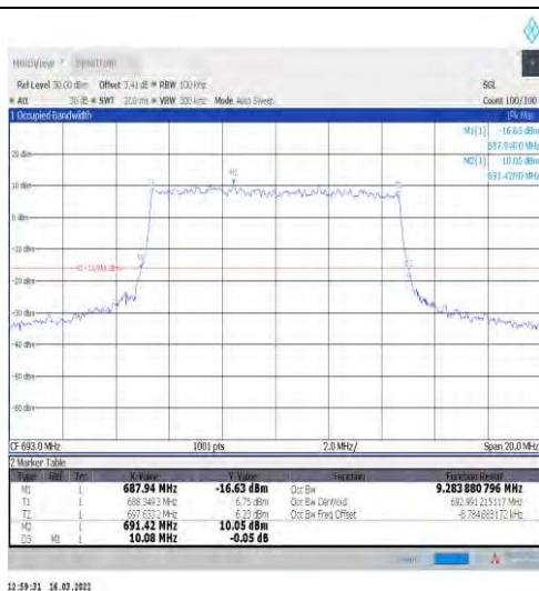
1-N71-15-10-H-8-CP-64QAM-Outer_Full-52@0-Ant1 -9.284-10.080≤10-PASS
