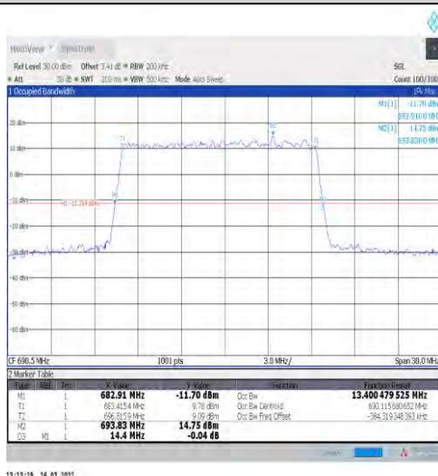
1-N71-15-15-H-3-DFT-16QAM-Outer_Full-75@0-Ant1 1-13.4-14.400≤15-PASS
