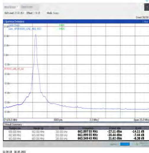
1-N71-15-20-L-1-DFT-PI2BPSK-Edge_1RB_Left-1@0-Ant1-PASS-see graph
