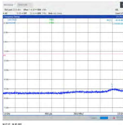
1-N71-15-20-L-1-DFT-PI2BPSK-Inner_1RB_Left-1@ 1-1000-3000-Ant1--48.40--13-PASS
