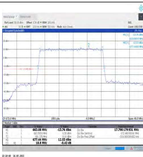
1-N71-15-20-L-4-DFT-64QAM-Outer_Full-100@0-An t1-17.79-18.800-<=20-PASS
