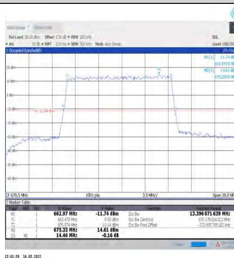
1-N71-15-15-L-2-DFT-PI2BPSK-Outer_Full-75@0-A nt1-13.396-14.460≤15-PASS
