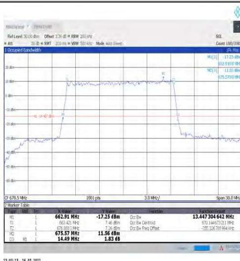
1-N71-15-15-L-5-DFT-256QAM-Outer_Full-75@0-Ant t1-13.447-14.490≤15-PASS
