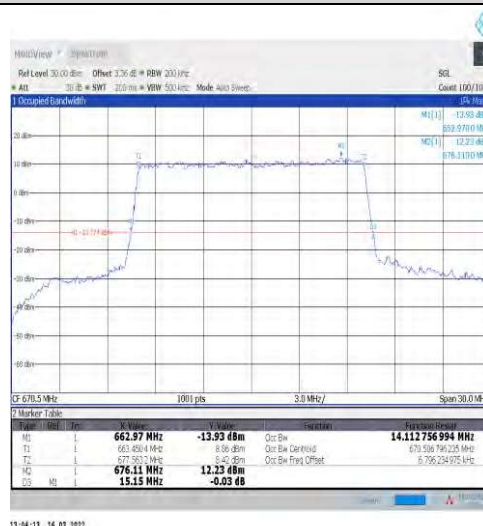
1-N71-15-15-L-6-CP-QPSK-Outer_Full-79@0-Ant1-1 4.113-15.150≤15-PASS
