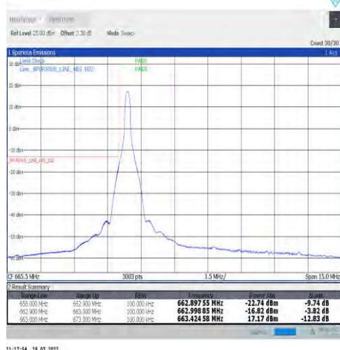
1-N71-15-10-L-4-CP-QPSK-Edge_1RB_Left-1@0-Ant1-PASS-see graph
