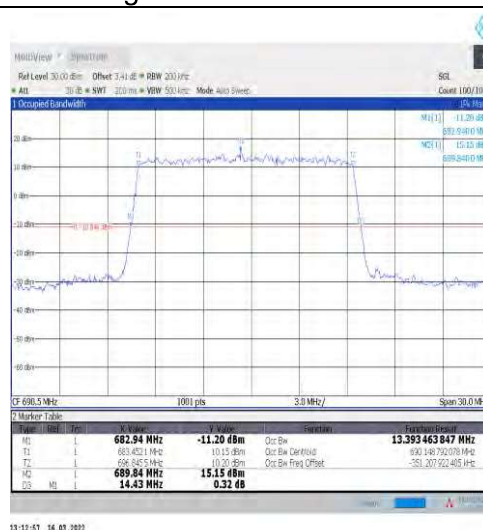
1-N71-15-15-H-2-DFT-PI2BPSK-Outer_Full-75@0-Ant1 -13.393-14.430≤15-PASS
