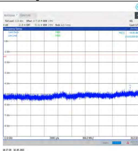
1-N71-15-20-L-1-DFT-PI2BPSK-Inner_1RB_Left-1@ 1-12000-20000-Ant1--44.86--13-PASS
