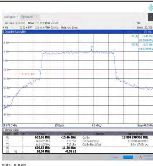
1-N71-15-20-L-6-CP-QPSK-Outer_Full-106@0-Ant1 -18.805-20.040-<=20-PASS
