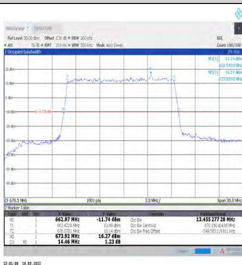
1-N71-15-15-L-1-DFT-QPSK-Outer_Full-75@0-Ant1- 13.455-14.460≤15-PASS
