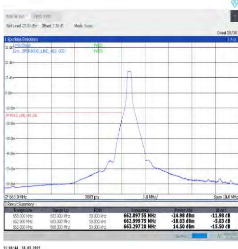
1-N71-15-5-L-4-CP-QPSK-Edge_1RB_Left-1@0-Ant1-PASS-see graph
