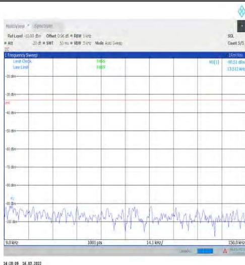
1-N71-15-20-M-1-DFT-PI2BPSK-Inner_1RB_Left-1@ 1-0.009-0.15-Ant1--90.51--33-PASS
