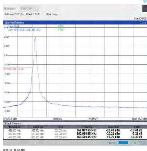
1-N71-15-20-L-4-CP-QPSK-Edge_1RB_Left-1@0-Ant1-PASS-see graph
