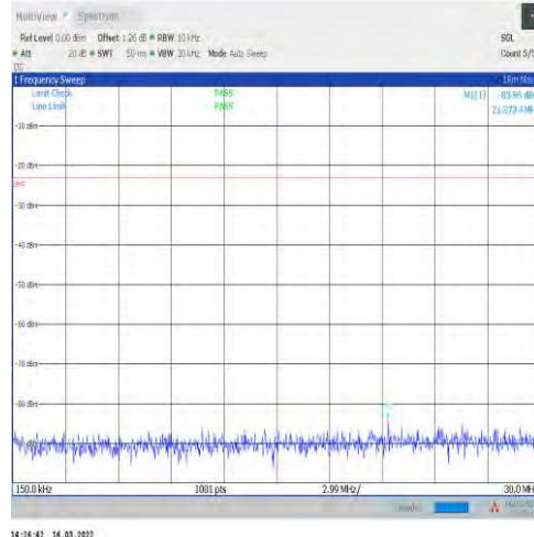
1-N71-15-20-L-1-DFT-PI2BPSK-Inner_1RB_Left-1@ 1-0.15-30-Ant1--83.86--23-PASS
