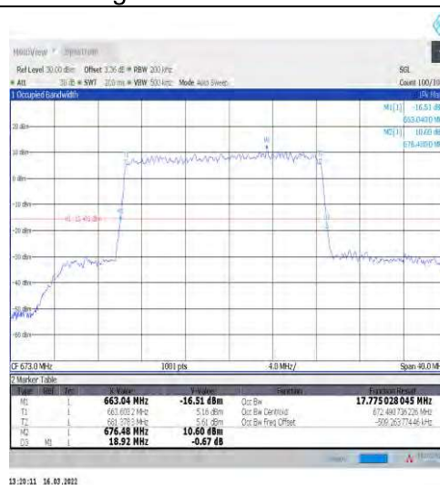
1-N71-15-20-L-5-DFT-256QAM-Outer_Full-100@0-A nt1-17.775-18.920-<=20-PASS
