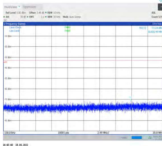
1-N77-3450-3550--30-100-L-1-DFT-QPSK-Edge_1R B_Left-1@0-0.15-30-Ant2--71.34--33-PASS
