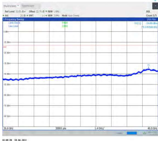
1-N77-3450-3550--30-100-L-1-DFT-QPSK-Edge_1R B_Left-1@0-26000-40000-Ant1--34.80--13-PASS
