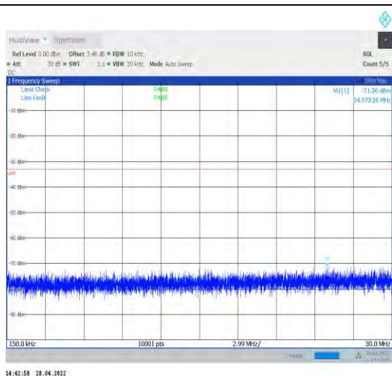
1-N77-3450-3550--30-100-M-1-DFT-QPSK-Edge_1R B_Left-1@0-0.15-30-Ant1--71.36--33-PASS
