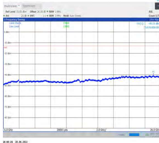
1-N77-3450-3550--30-100-L-1-DFT-QPSK-Edge_1R B_Left-1@0-6000-26000-Ant2--40.31--13-PASS
