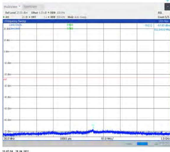
1-N77-3450-3550--30-100-L-1-DFT-QPSK-Edge_1R B_Left-1@0-30-1000-Ant1--67.85--23-PASS
