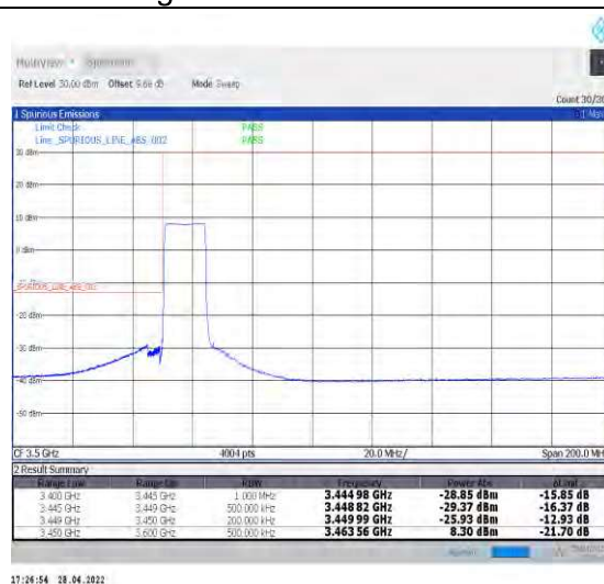
1-N77-3450-3550--30-15-L-6-CP-QPSK-Outer_Ful l-38@0-Ant2-PASS-see graph
