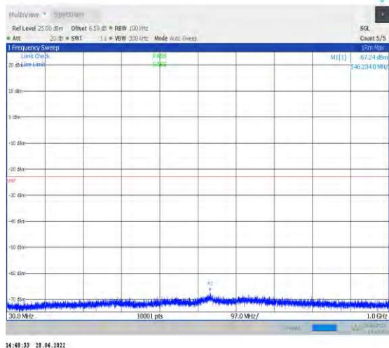
1-N77-3450-3550--30-100-H-1-DFT-QPSK-Edge_1R B_Left-1@0-30-1000-Ant2--67.24--23-PASS
