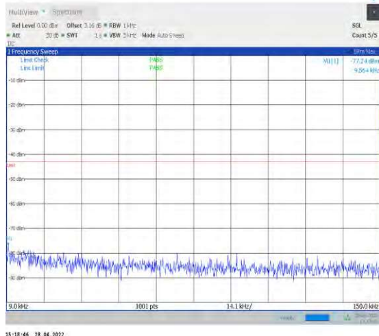
1-N77-3450-3550--30-100-L-1-DFT-QPSK-Edge_1R B_Left-1@0-0.009-0.15-Ant1--77.24--43-PASS
