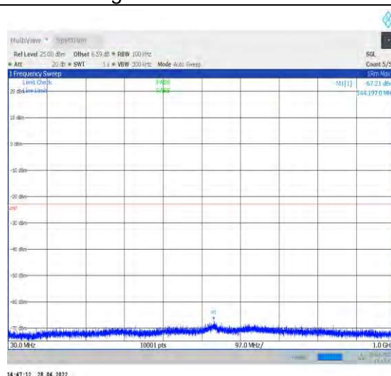
1-N77-3450-3550--30-100-M-1-DFT-QPSK-Edge_1R B_Left-1@0-30-1000-Ant2--67.21--23-PASS
