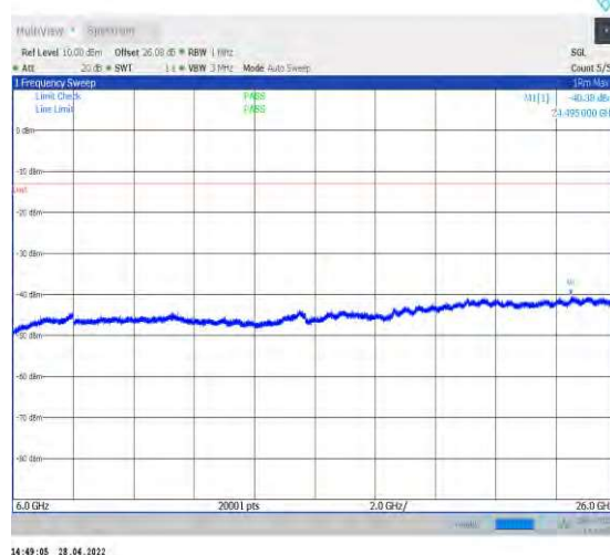
1-N77-3450-3550--30-100-H-1-DFT-QPSK-Edge_1R B_Left-1@0-6000-26000-Ant2--40.38--13-PASS
