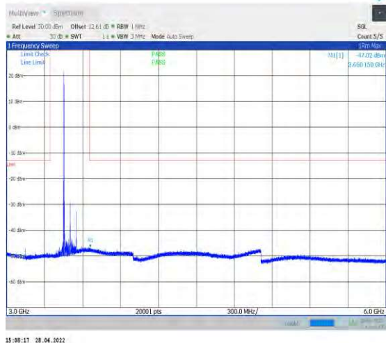
1-N77-3450-3550--30-100-L-1-DFT-QPSK-Edge_1R B_Left-1@0-3000-6000-Ant1--47.02--13-PASS
