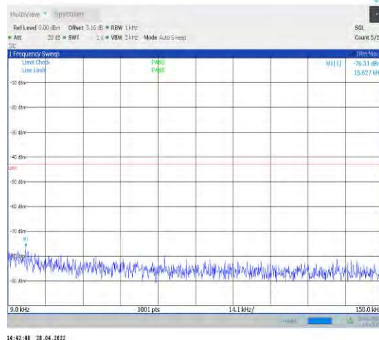
1-N77-3450-3550--30-100-M-1-DFT-QPSK-Edge_1R B_Left-1@0-0.009-0.15-Ant1--76.51--43-PASS
