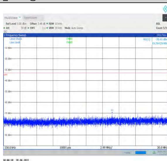
1-N77-3450-3550--30-100-H-1-DFT-QPSK-Edge_1R B_Left-1@0-0.15-30-Ant1--70.41--33-PASS
