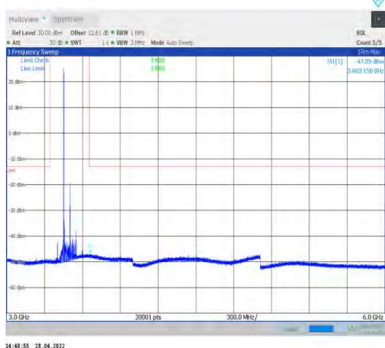
1-N77-3450-3550--30-100-H-1-DFT-QPSK-Edge_1R B_Left-1@0-3000-6000-Ant2--47.09--13-PASS
