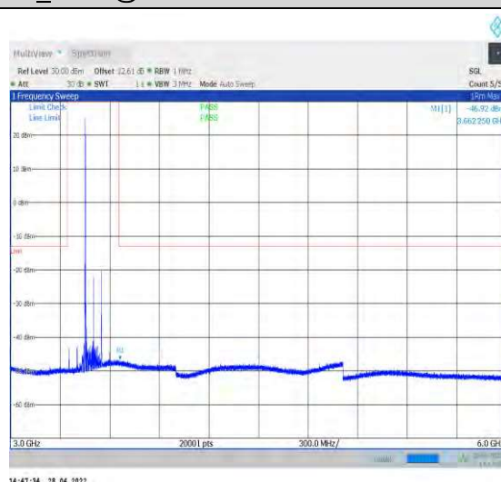
1-N77-3450-3550--30-100-M-1-DFT-QPSK-Edge_1R B_Left-1@0-3000-6000-Ant2--46.92--13-PASS
