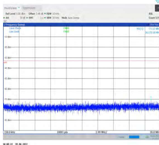
1-N77-3450-3550--30-100-H-1-DFT-QPSK-Edge_1R B_Left-1@0-0.15-30-Ant2--71.12--33-PASS
