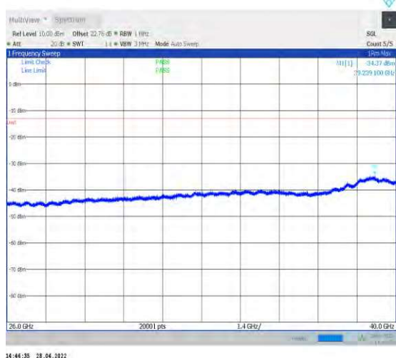
1-N77-3450-3550--30-100-L-1-DFT-QPSK-Edge_1R B_Left-1@0-26000-40000-Ant2--34.37--13-PASS
