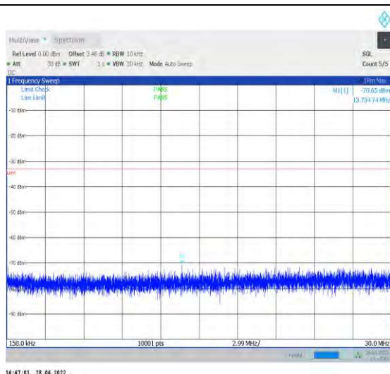
1-N77-3450-3550--30-100-M-1-DFT-QPSK-Edge_1R B_Left-1@0-0.15-30-Ant2--70.65--33-PASS
