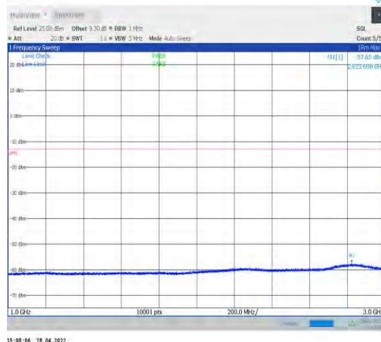
1-N77-3450-3550--30-100-L-1-DFT-QPSK-Edge_1R B_Left-1@0-1000-3000-Ant1--57.65--13-PASS
