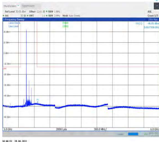
1-N77-3450-3550--30-100-H-1-DFT-QPSK-Edge_1R B_Left-1@0-3000-6000-Ant1--46.93--13-PASS
