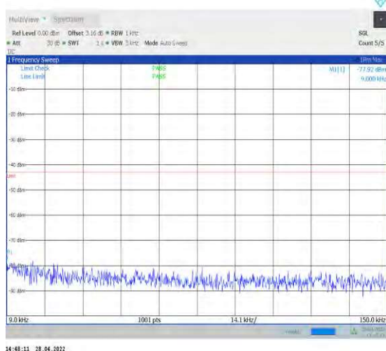
1-N77-3450-3550--30-100-H-1-DFT-QPSK-Edge_1R B_Left-1@0-0.009-0.15-Ant2--77.92--43-PASS
