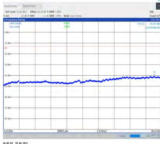
1-N77-3450-3550--30-100-H-1-DFT-QPSK-Edge_1R B_Left-1@0-6000-26000-Ant1--39.95--13-PASS
