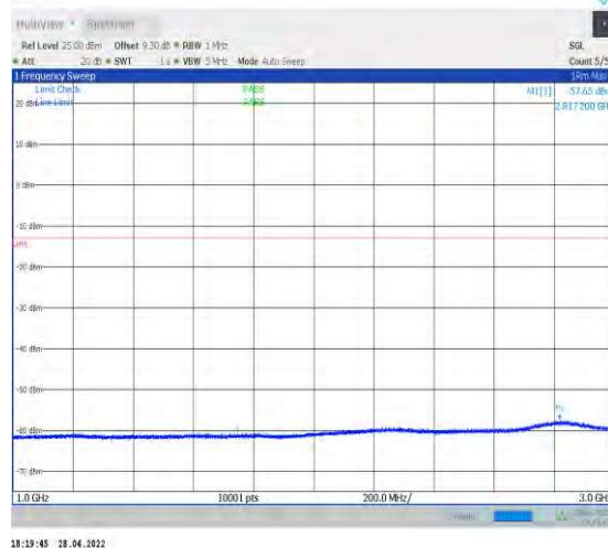
1-N77-3700-3980--30-100-L-1-DFT-QPSK-Edge_1R B_Left-1@0-1000-3000-Ant1--57.65--13-PASS
