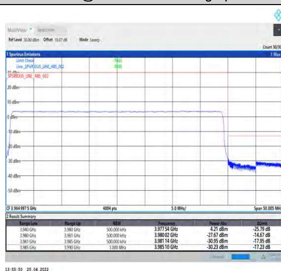
1-N77-3700-3980--30-40-H-6-CP-QPSK-Outer_Full-1@106@0-Ant2-PASS-see graph
