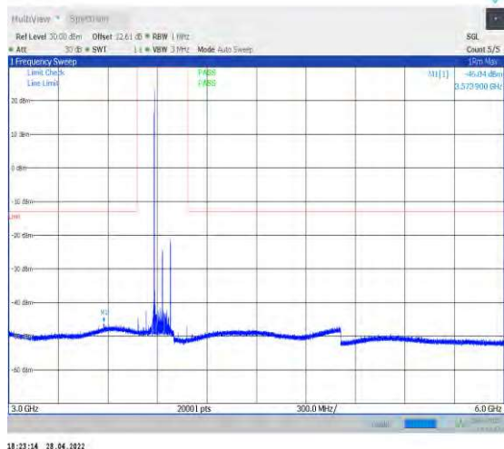
1-N77-3700-3980--30-100-H-1-DFT-QPSK-Edge_1R B_Left-1@0-3000-6000-Ant1--46.04--13-PASS
