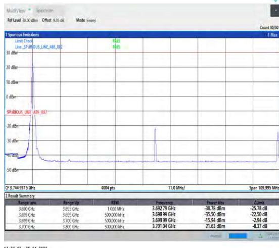
1-N77-3700-3980--30-100-L-4-CP-QPSK-Edge_1RB_L eft-1@0-Ant2-PASS-see graph
