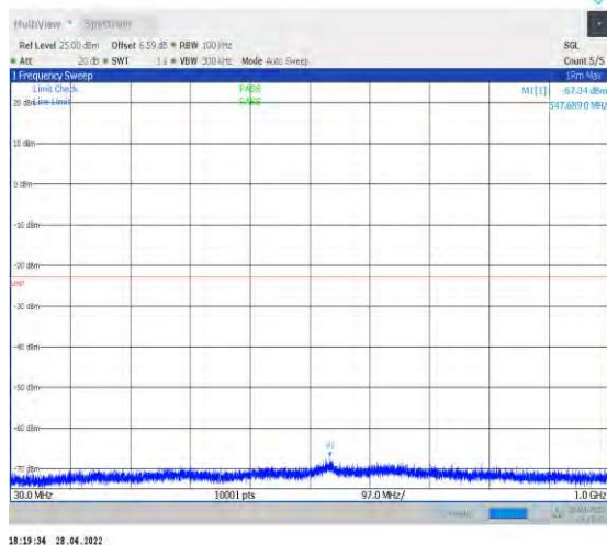
1-N77-3700-3980--30-100-L-1-DFT-QPSK-Edge_1R B_Left-1@0-30-1000-Ant1--67.34--23-PASS
