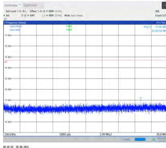
1-N77-3700-3980--30-100-L-1-DFT-QPSK-Edge_1R B_Left-1@0-0.15-30-Ant1--71.02--33-PASS
