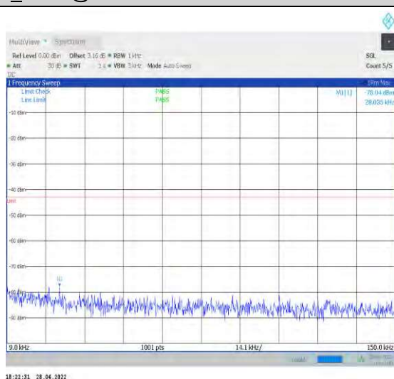
1-N77-3700-3980--30-100-H-1-DFT-QPSK-Edge_1R B_Left-1@0-0.009-0.15-Ant1--78.04--43-PASS
