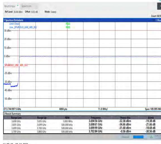
1-N77-3700-3980--30-100-L-6-CP-QPSK-Outer_F ull-273@0-Ant2-PASS-see graph
