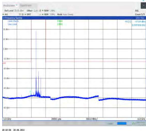
1-N77-3700-3980--30-100-L-1-DFT-QPSK-Edge_1R B_Left-1@0-3000-6000-Ant1--47.04--13-PASS
