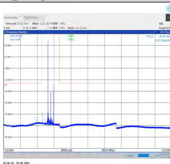
1-N77-3700-3980--30-100-M-1-DFT-QPSK-Edge_1R B_Left-1@0-3000-6000-Ant2--46.35--13-PASS
