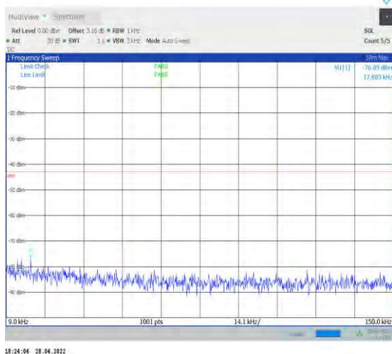
1-N77-3700-3980--30-100-L-1-DFT-QPSK-Edge_1R B_Left-1@0-0.009-0.15-Ant2--76.89--43-PASS
