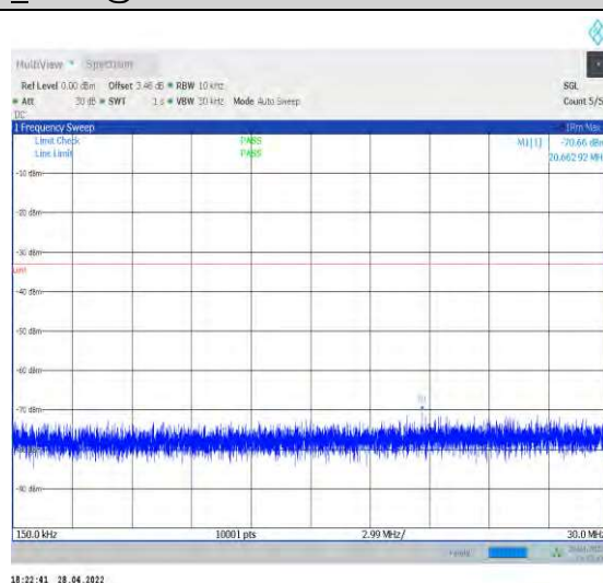
1-N77-3700-3980--30-100-H-1-DFT-QPSK-Edge_1R B_Left-1@0-0.15-30-Ant1--70.66--33-PASS
