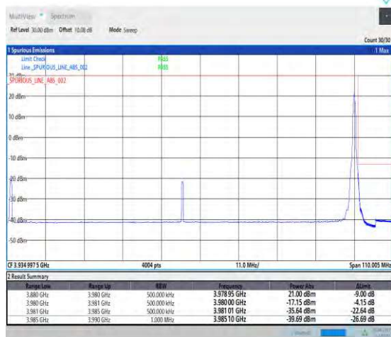
1-N77-3700-3980--30-100-H-5-CP-QPSK-Edge_1RB_ Right-1@272-Ant2-PASS-see graph
