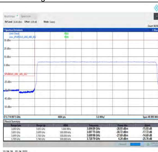
1-N77-3700-3980--30-40-L-6-CP-QPSK-Outer_Ful I-106@0-Ant2-PASS-see graph
