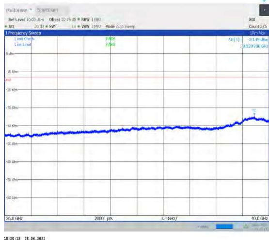
1-N77-3700-3980--30-100-L-1-DFT-QPSK-Edge_1R B_Left-1@0-26000-40000-Ant1--34.49--13-PASS
