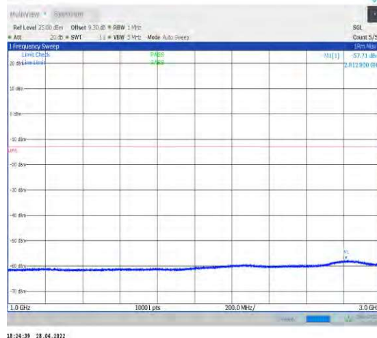
1-N77-3700-3980--30-100-L-1-DFT-QPSK-Edge_1R B_Left-1@0-1000-3000-Ant2--57.71--13-PASS
