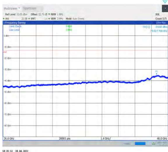
1-N77-3700-3980--30-100-L-1-DFT-QPSK-Edge_1R B_Left-1@0-26000-40000-Ant2--34.85--13-PASS
