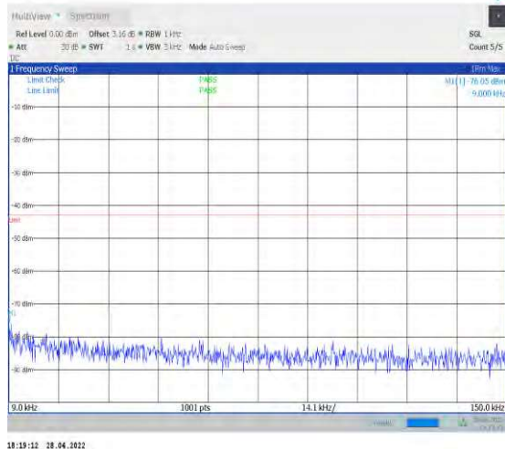
1-N77-3700-3980--30-100-L-1-DFT-QPSK-Edge_1R B_Left-1@0-0.009-0.15-Ant1--76.05--43-PASS
