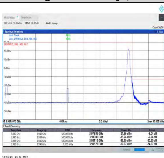
1-N77-3700-3980--30-40-H-5-CP-QPSK-Edge_1RB_Right-1@105-Ant2-PASS-see graph
