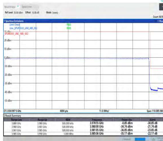
1-N77-3700-3980--30-100-H-6-CP-QPSK-Outer_F ull-273@0-Ant2-PASS-see graph
