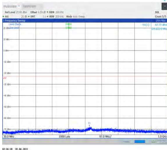
1-N77-3700-3980--30-100-L-1-DFT-QPSK-Edge_1R B_Left-1@0-30-1000-Ant2--67.75--23-PASS
