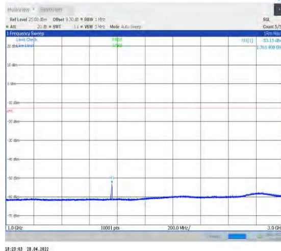
1-N77-3700-3980--30-100-H-1-DFT-QPSK-Edge_1R B_Left-1@0-1000-3000-Ant1--53.15--13-PASS
