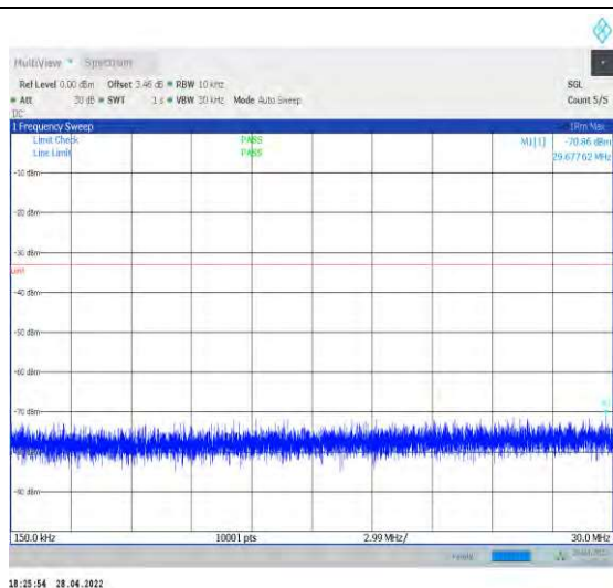
1-N77-3700-3980--30-100-M-1-DFT-QPSK-Edge_1R B_Left-1@0-0.15-30-Ant2--70.86--33-PASS
