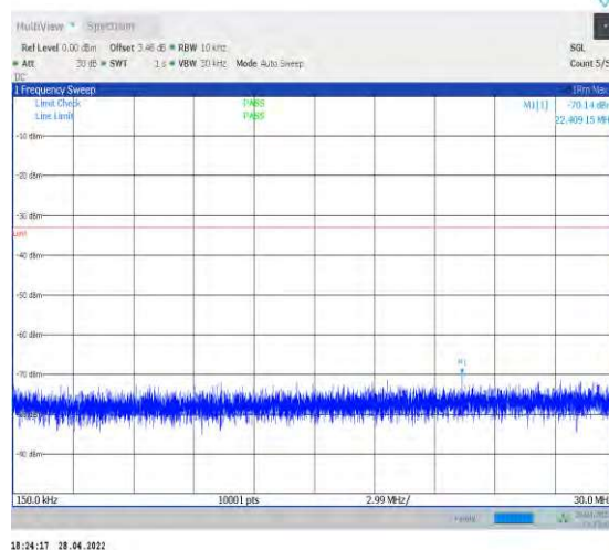
1-N77-3700-3980--30-100-L-1-DFT-QPSK-Edge_1R B_Left-1@0-0.15-30-Ant2--70.14--33-PASS
