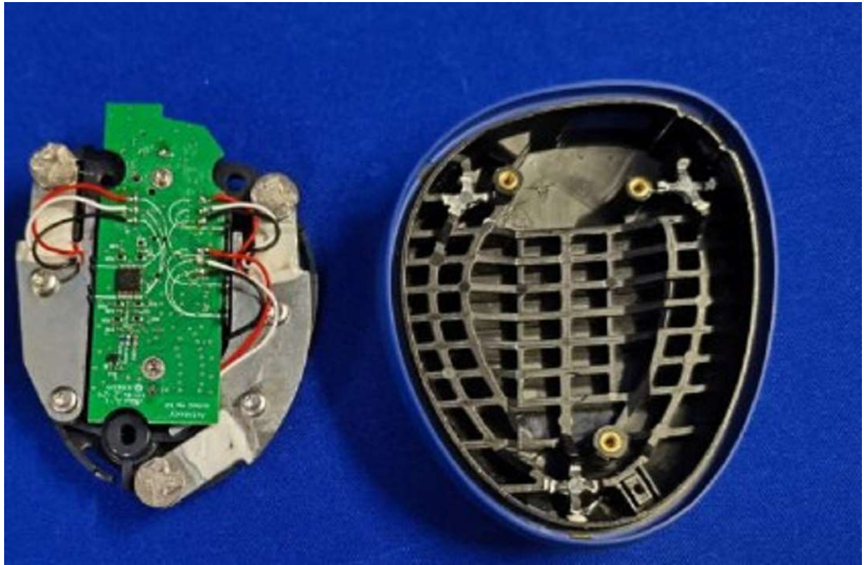
Device Open 2
