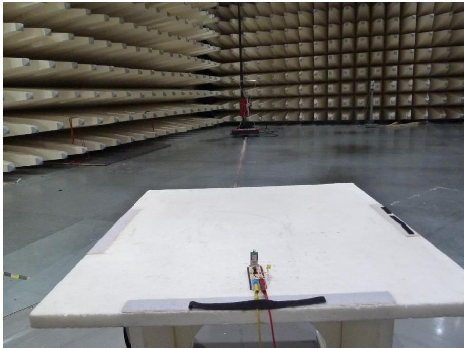
Photo 4 (RSE set-up / Semi-anechoic chamber):
