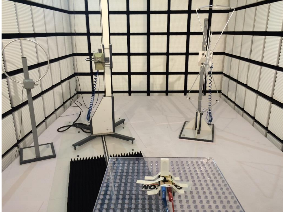
Photo 3 (RSE set-up / fully-anechoic chamber):
