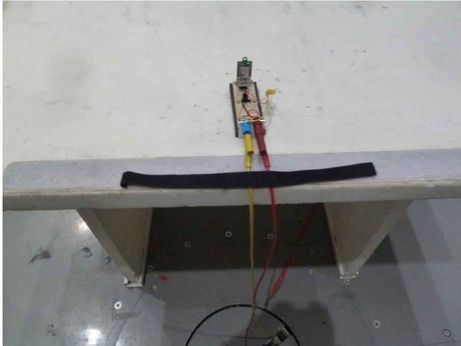
Photo 5 (RSE set-up / Semi-anechoic chamber):
