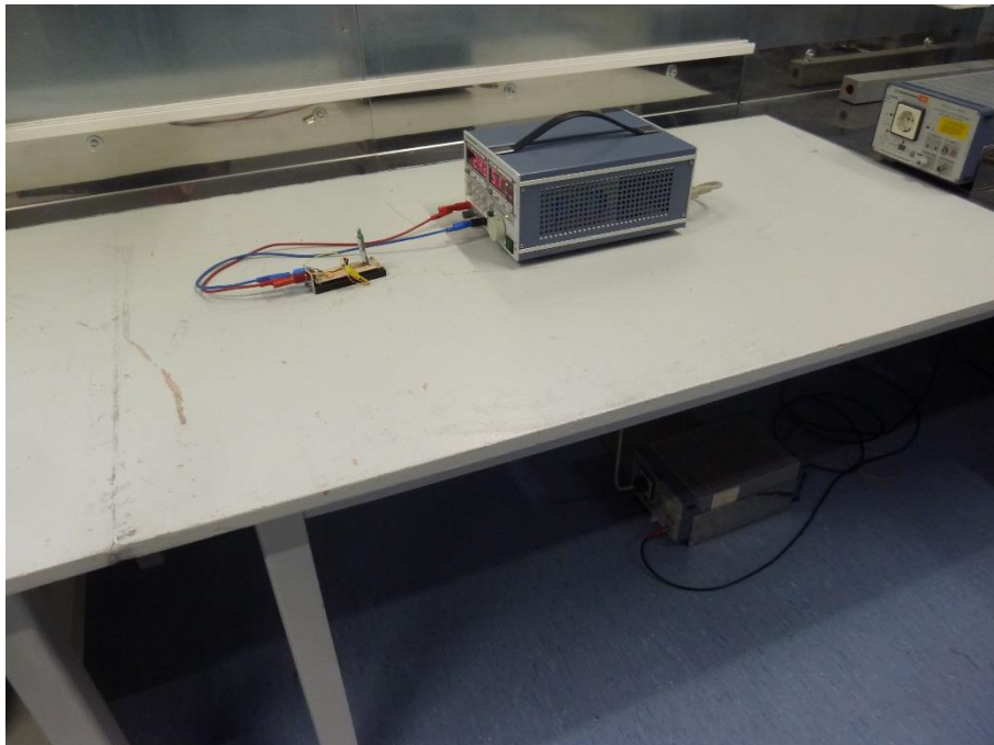
Photo 6 (AC Emissions):
