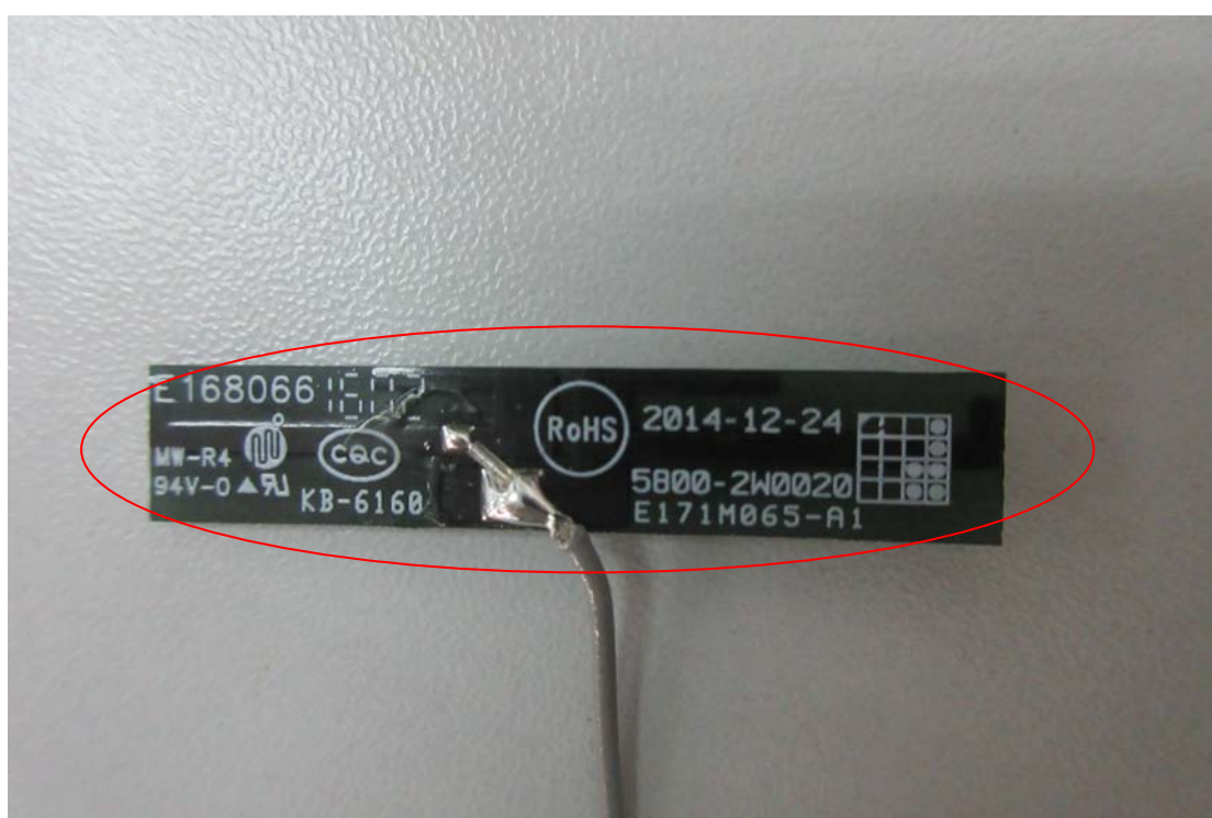
8. 5G antenna 2 view and 2.4G antenna 1 view
