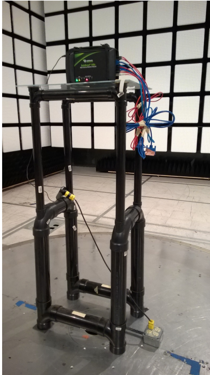
Figure 3.6-1: Setup Photo – Radiated Emissions > 1GHz
