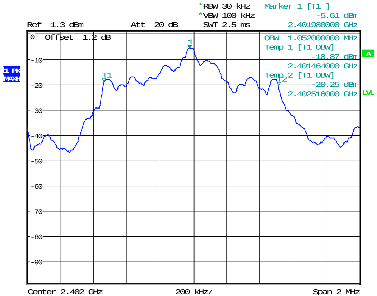
Plot 1. 4 - 99% Bandwidth
