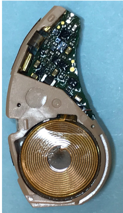
Processor PCBA Back 2
