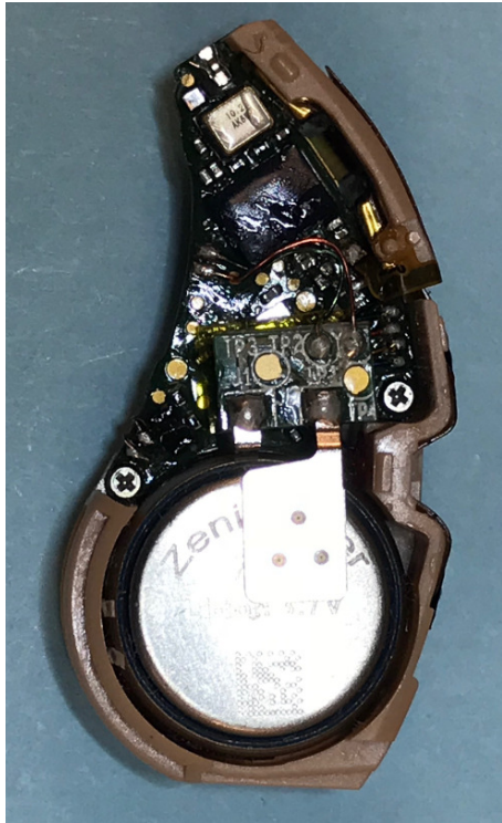
Processor PCBA Front 1
