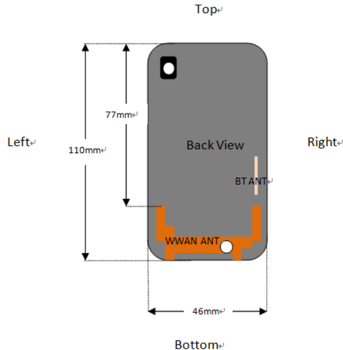
Fig.14.1 EUT Antenna Locations
