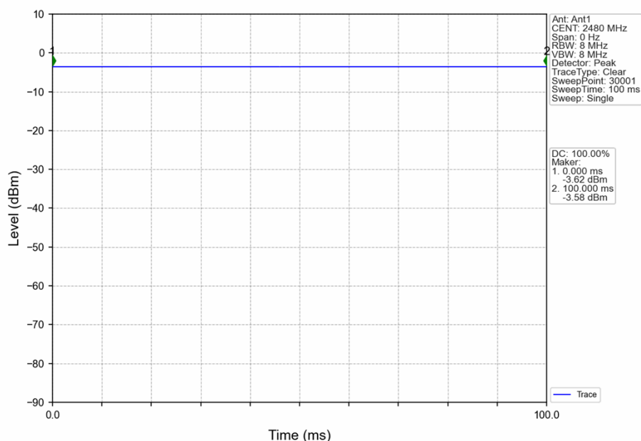
1M_HCH_2480MHz_Ant1_NTNV
