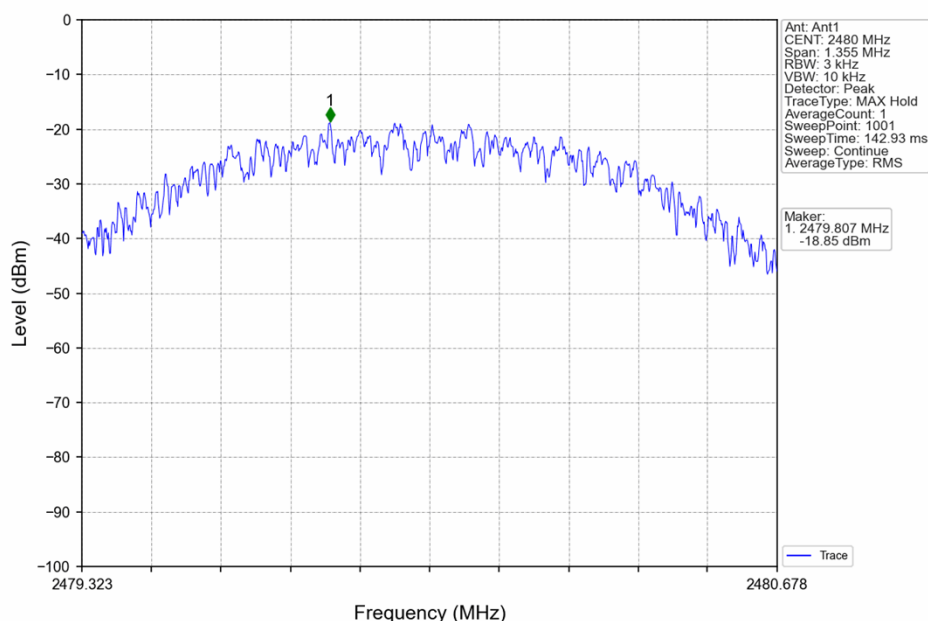
1M_HCH_2480MHz_Ant1_NTNV
