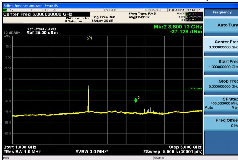
Band41-10MHz-QPSK-40740-1RB#0-Range5:5000~12000MHz
