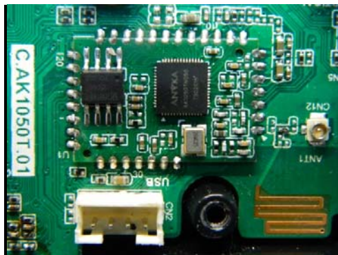
Antenna 2
