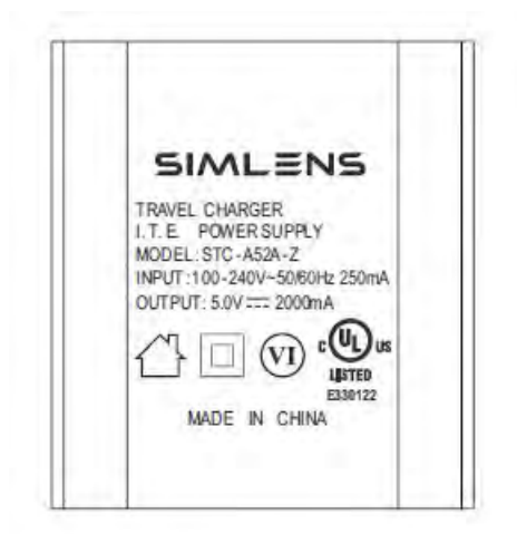
THE LABEL OF CHARGER
