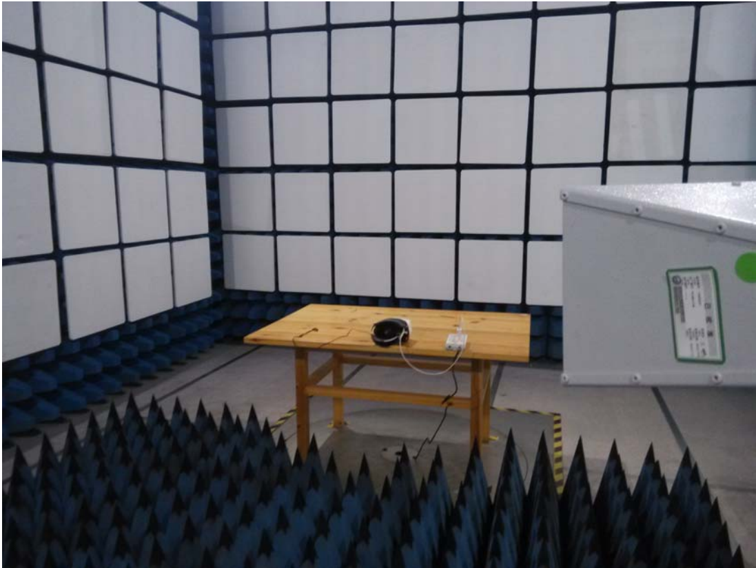
Above 1 GHz, The Charge (Adapter) test mode
