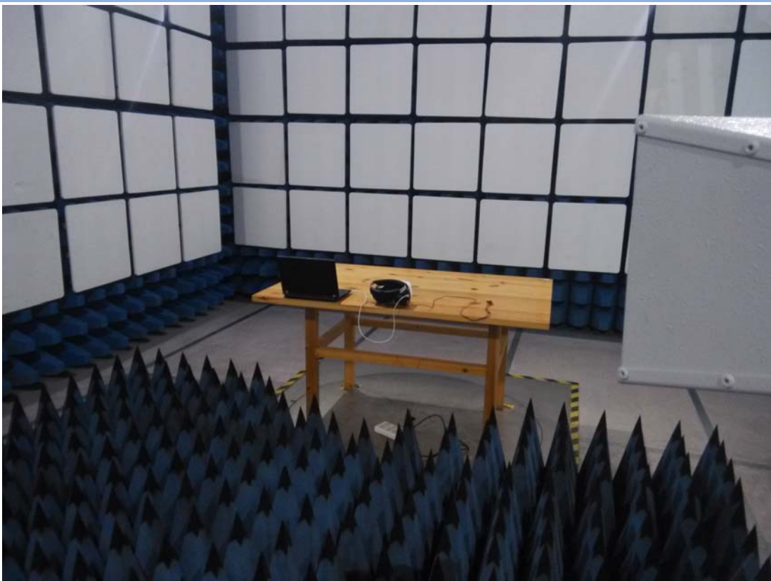
Above 1 GHz, The Data Transfer test mode
