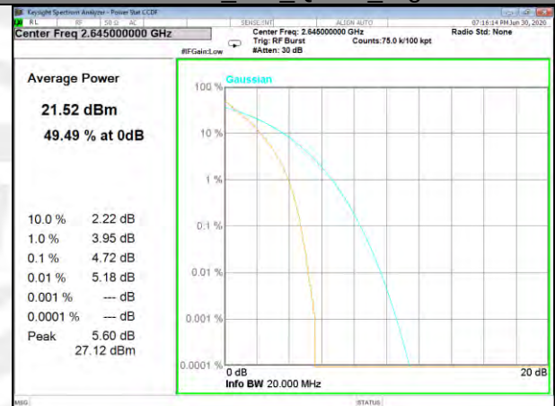
Band41_100_Q16_High
