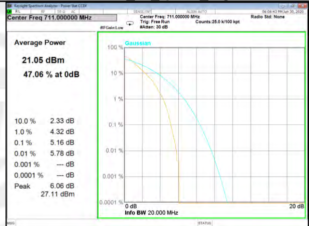
Band12_50_Q16_High
