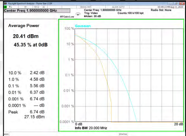
Band2_100_Q16_High
