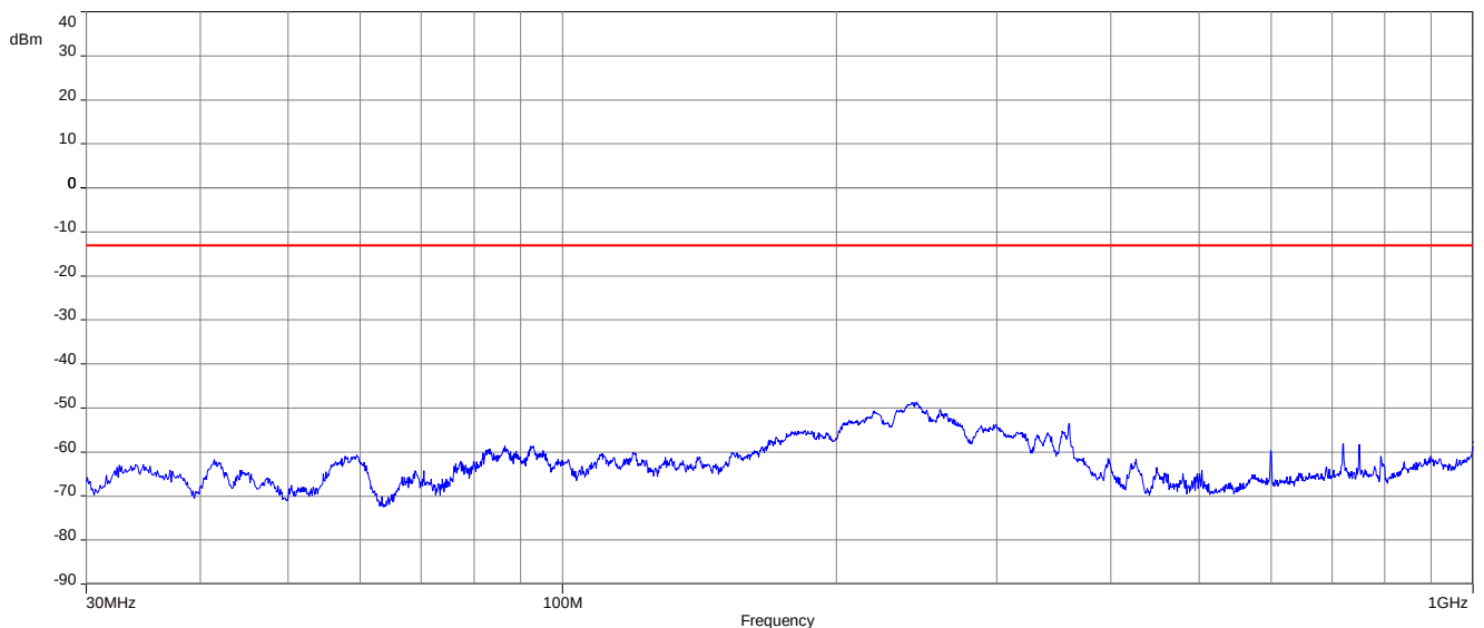
Plot 2: Channel 132322 (30 MHz – 1 GHz)
