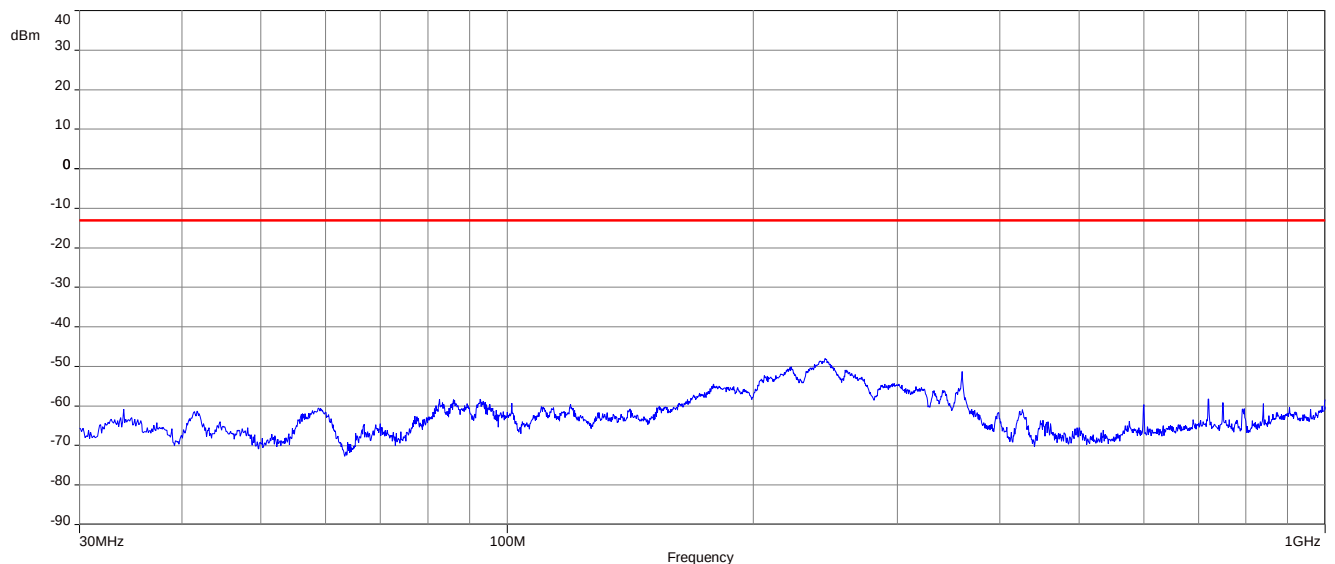
Plot 2: Channel 26340 (30 MHz – 1 GHz)
