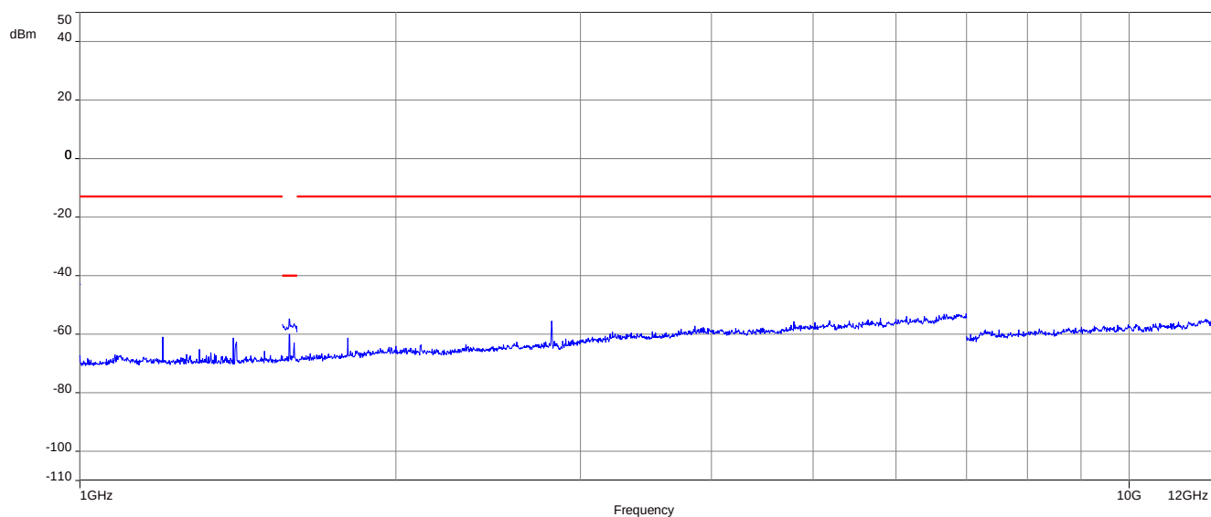
Plot 3: channel 23095 (1 GHz to 12 GHz)
