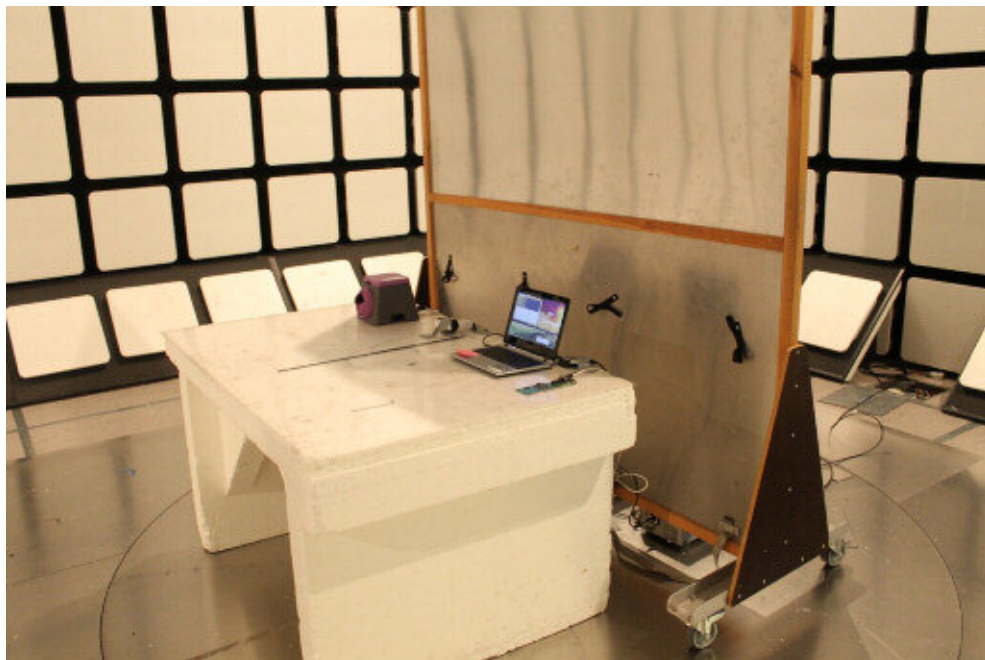
Photograph 4. The EUT and test set-up for conducted emission test.
