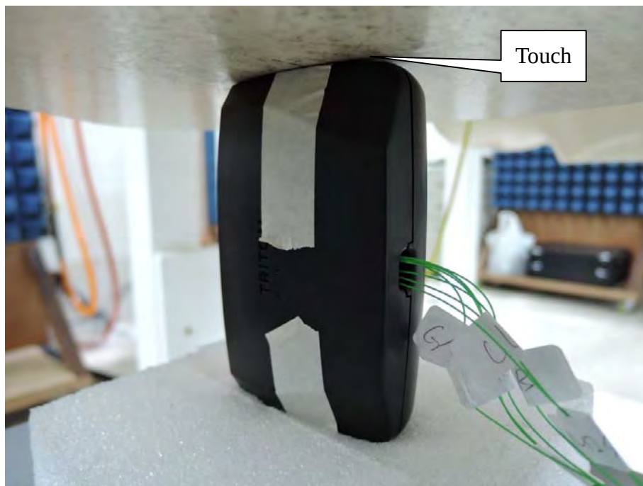
EUT Right-Side (BLE)
