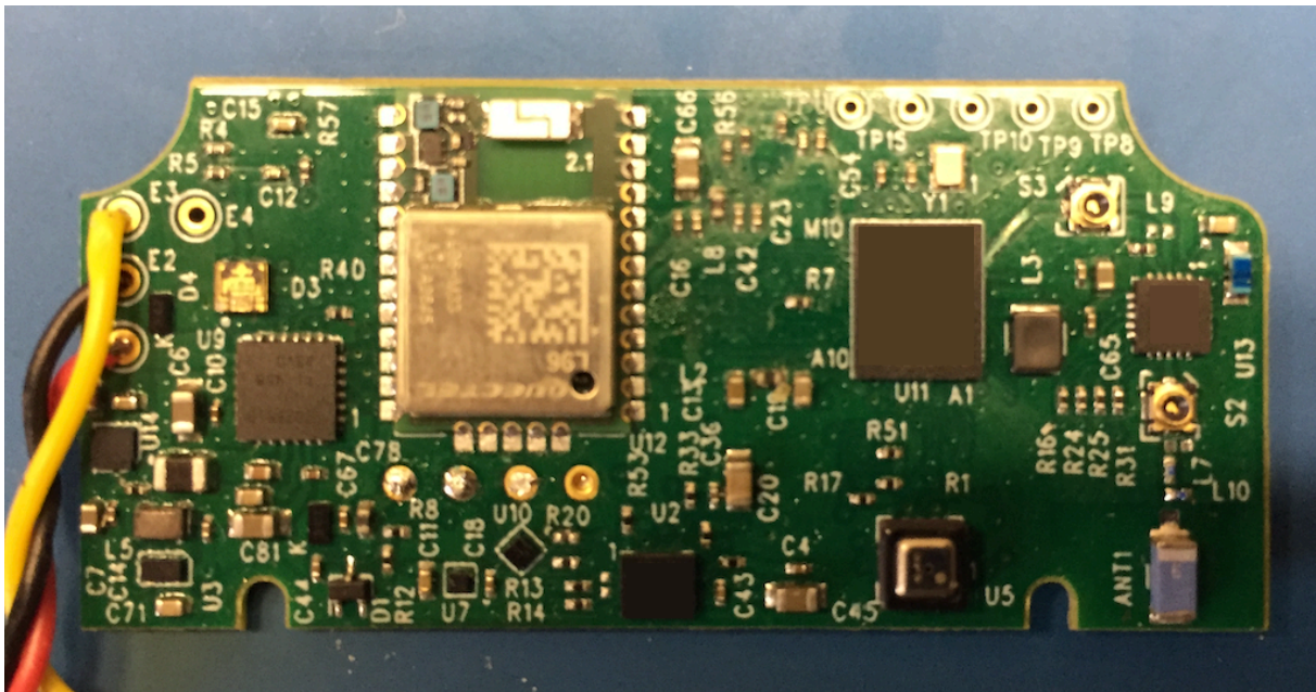
Board Top Side
