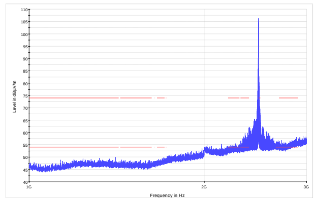
Figure 8.7-11: Radiated spurious emissions within 1–3 GHz, high channel
