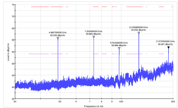
Figure 8.7-13: Radiated spurious emissions within 3–18 GHz, mid channel
