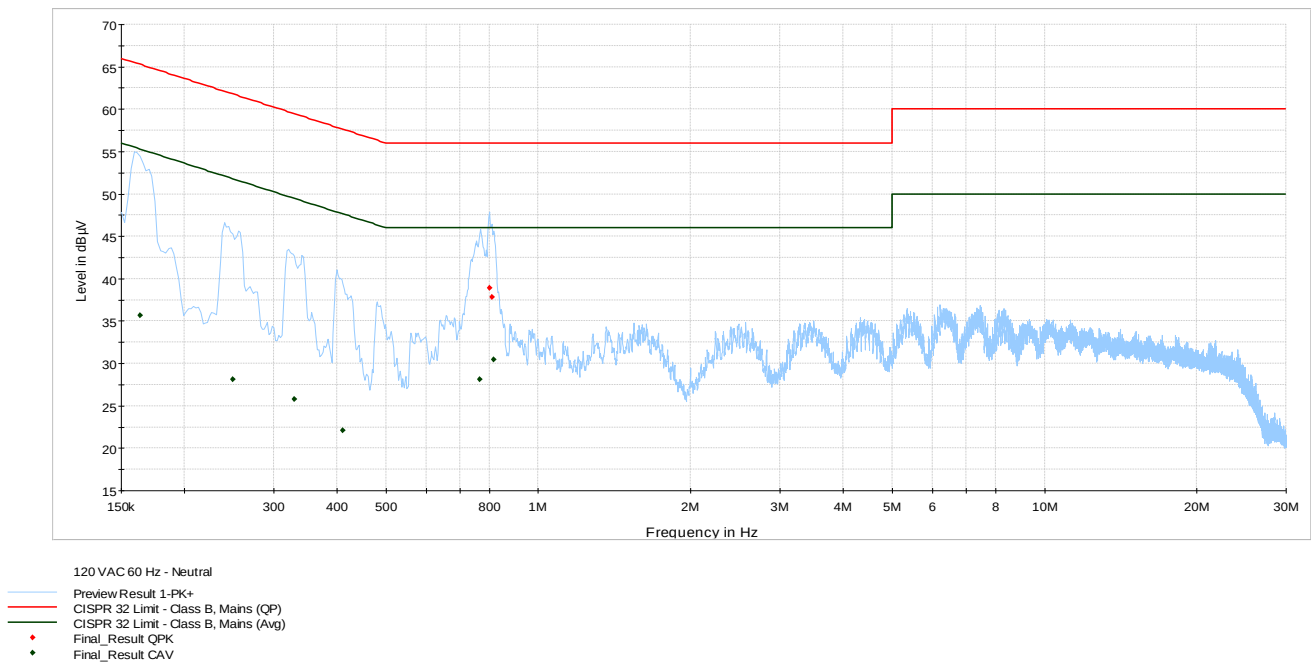
Plot 8.4-2: Conducted emissions on neutral line
