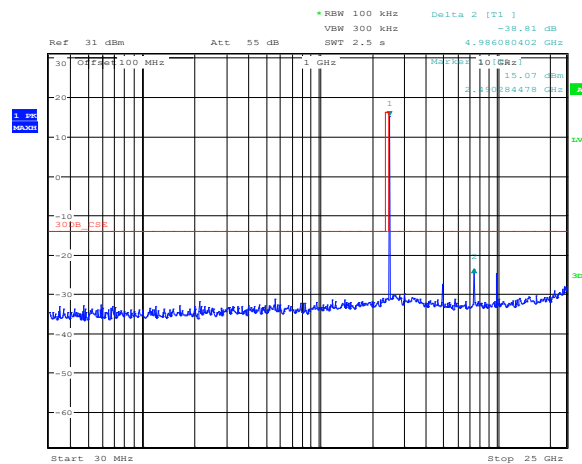
Figure 8.7-3: Conducted spurious emissions, low channel
