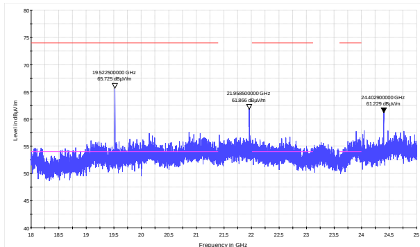
Figure 8.7-16: Radiated spurious emissions above 18 GHz, mid channel
