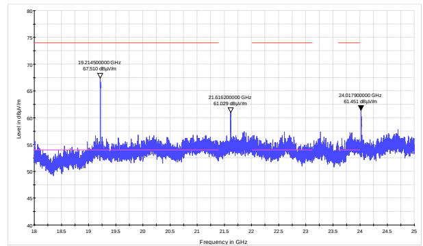
Figure 8.7-15: Radiated spurious emissions above 18 GHz, low channel
