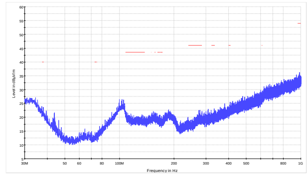
Figure 8.7-7: Radiated spurious emissions below 1 GHz, mid channel
