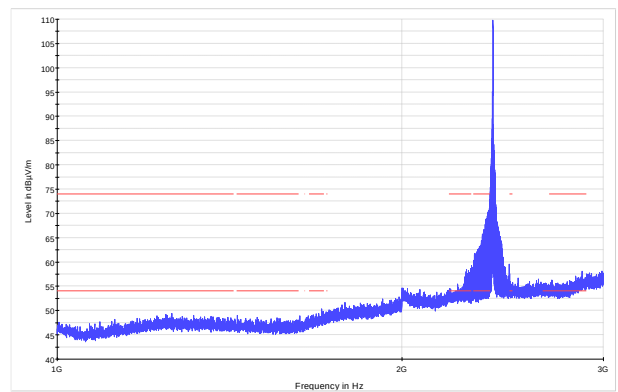
Figure 8.7-9: Radiated spurious emissions within 1–3 GHz, low channel
