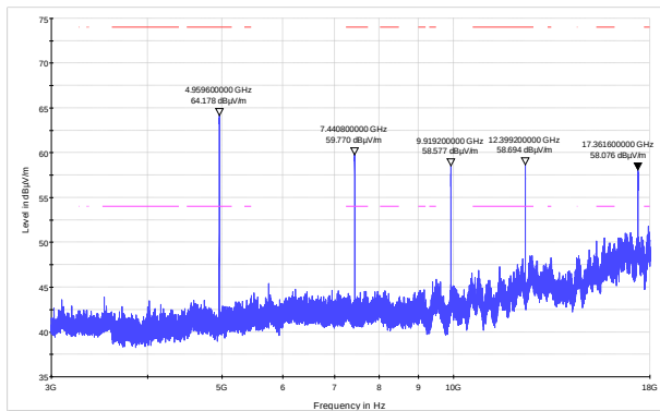
Figure 8.7-14: Radiated spurious emissions within 3–18 GHz, high channel
