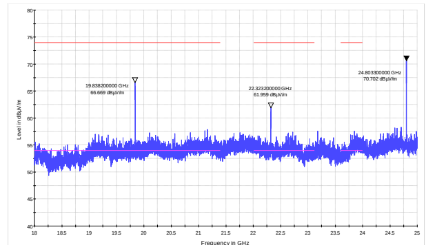
Figure 8.7-17: Radiated spurious emissions above 18 GHz, high channel
