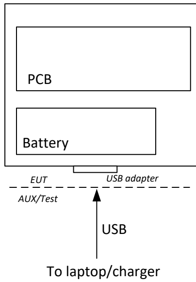
Figure 3.6-1: Setup diagram
