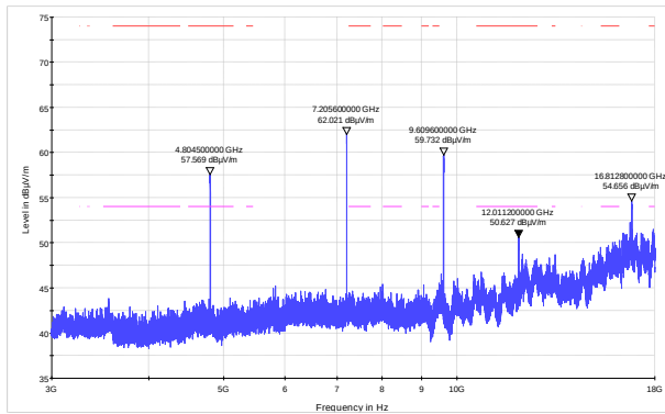
Figure 8.7-12: Radiated spurious emissions within 3–18 GHz, low channel
