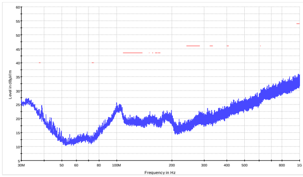
Figure 8.7-6: Radiated spurious emissions below 1 GHz, low channel
