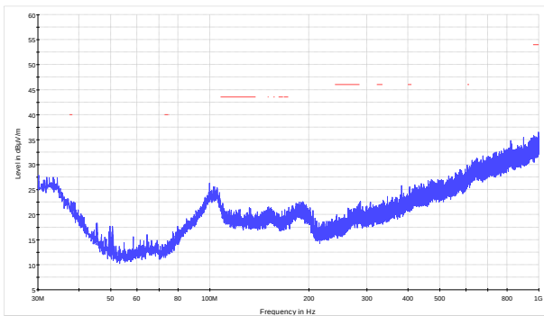
Figure 8.7-8: Radiated spurious emissions below 1 GHz, high channel
