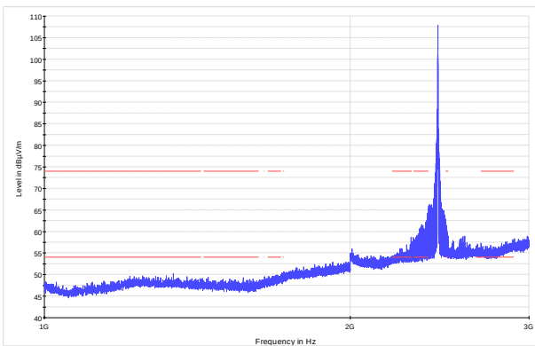
Figure 8.7-10: Radiated spurious emissions within 1–3 GHz, mid channel
