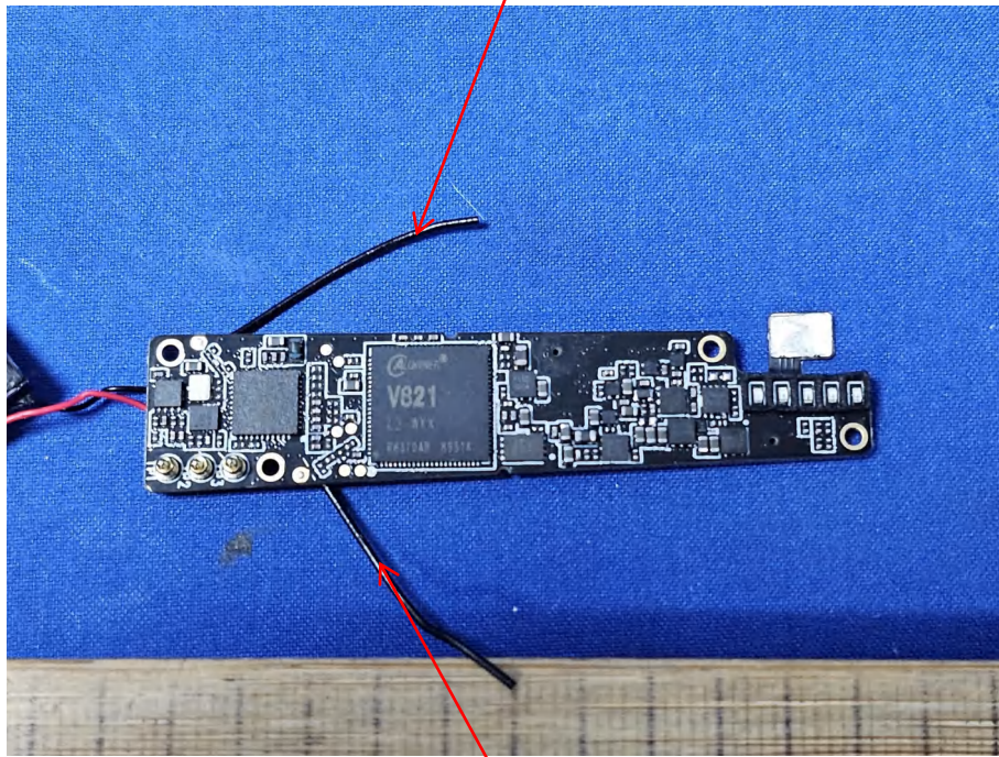
WLAN Antenna
