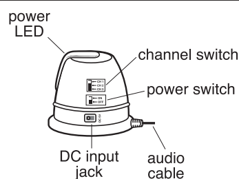
signal transmitter
