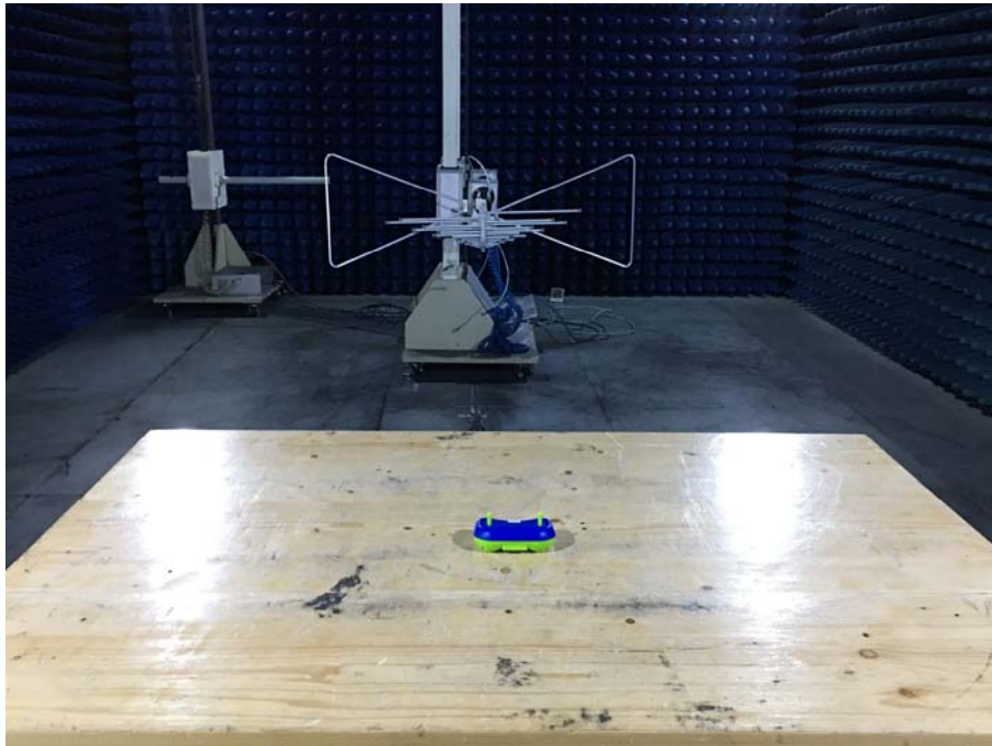
Photograph of set-up for Radiated Emission
