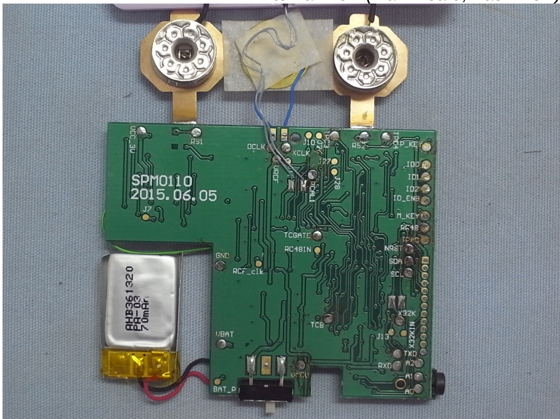
Internal View (Main Board, Back View)
