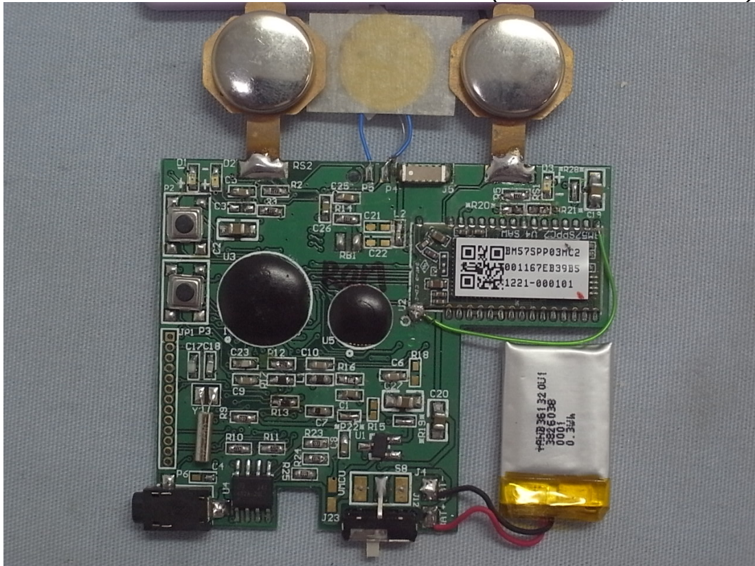
Internal View (Main Board, Front View)
