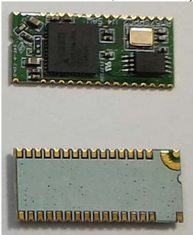
Figure 8 Internal View (RF Module Board Removed Cover, Front Back View)
