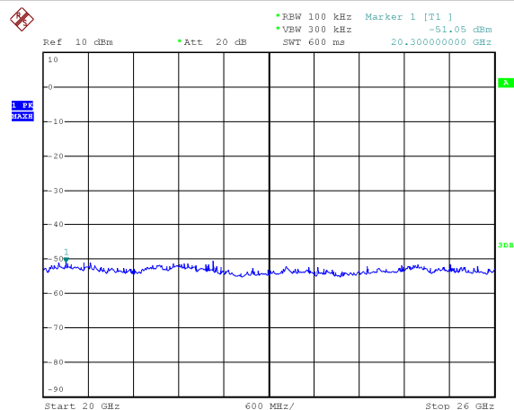
Plot 6 (20÷26GHz)
