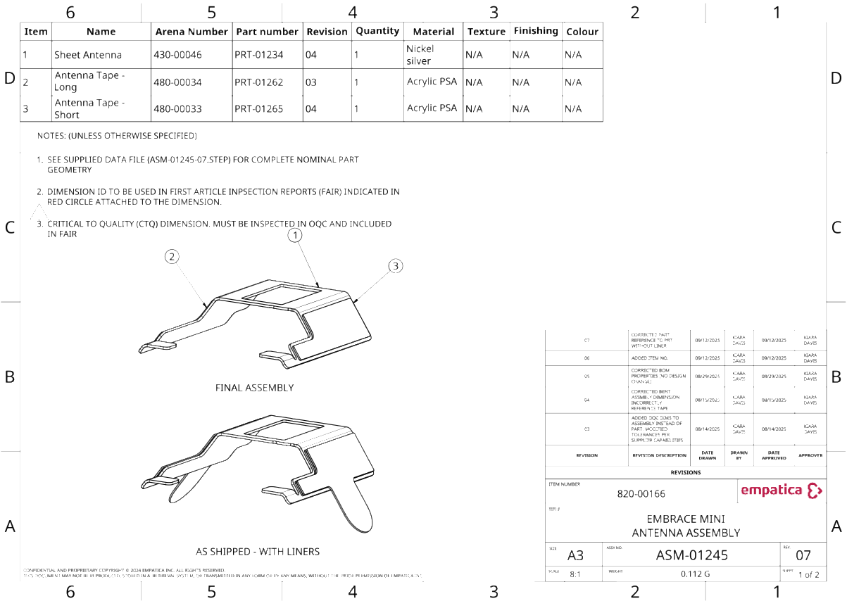
Figure 1 - Technical Drawing of the antenna
