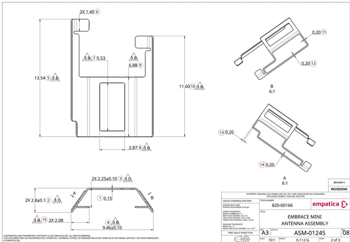
Figure 2 - Antenna drawing with dimensions
