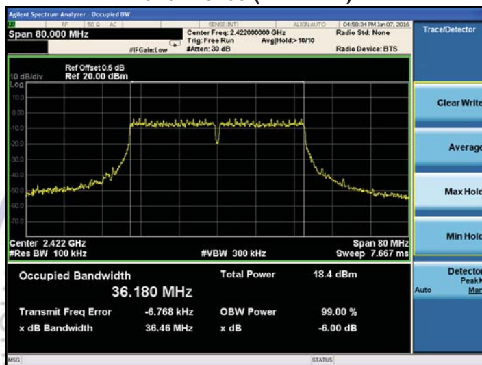
Channel 03 (2422MHz)
