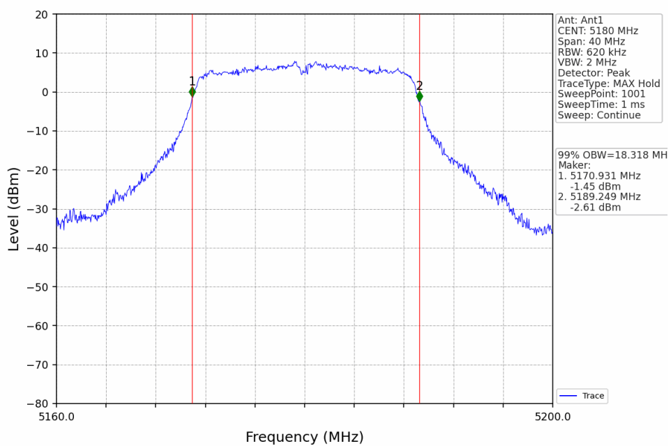
802.11ac(VHT20)_LCH_5180MHz_Ant1_NTNV
