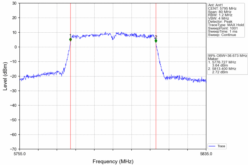
802.11ac(VHT40)_HCH_5795MHz_Ant2_NTNV
