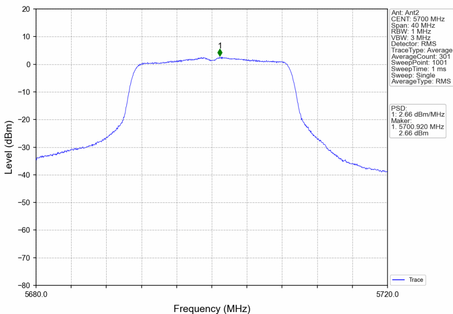
802.11n(HT20)_HCH_5700MHz_MIMO_NTNV
