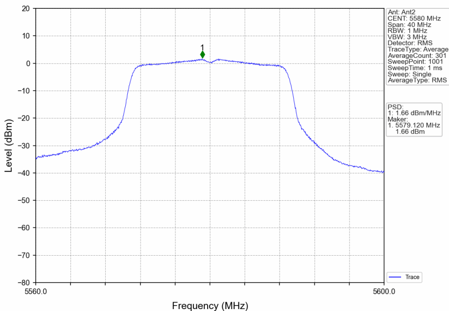
802.11n(HT20)_MCH_5580MHz_Ant2_NTNV
