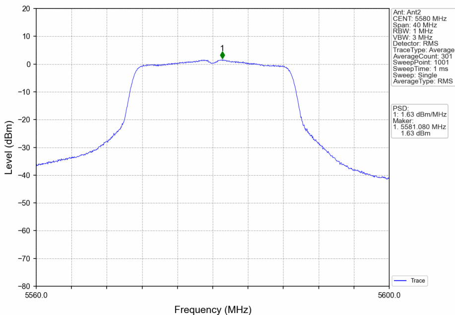
802.11ac(VHT20)_MCH_5580MHz_Ant2_NTNV
