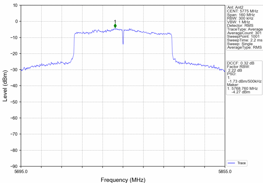
802.11ac(VHT80)_MCH_5775MHz_MIMO_NTNV
