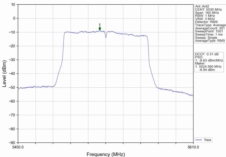
802.11ac(VHT80)_LCH_5530MHz_MIMO_NTNV
