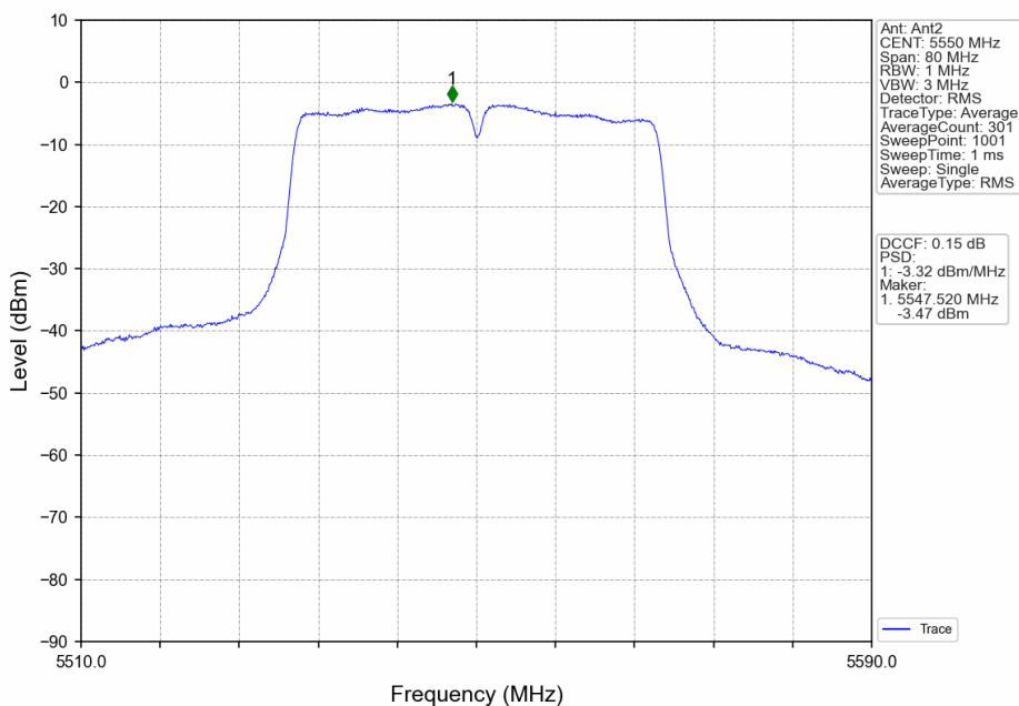
802.11ac(VHT40)_MCH_5550MHz_MIMO_NTNV
