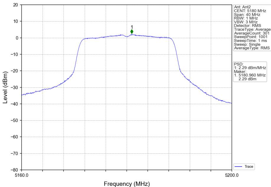
802.11ac(VHT20)_LCH_5180MHz_MIMO_NTNV
