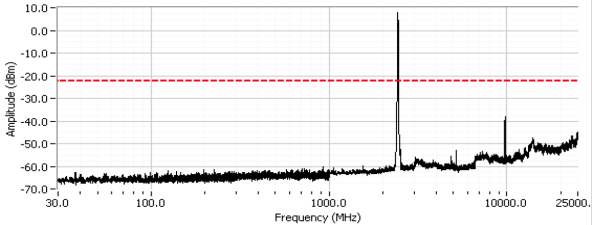
802.11n40, 2437 MHz
