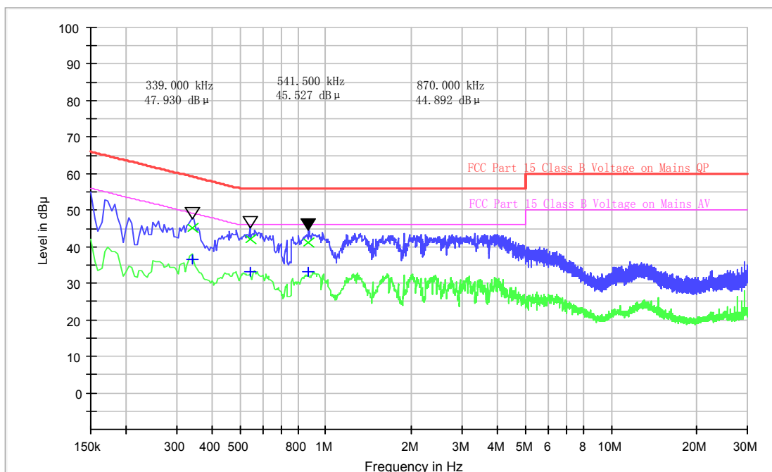
FCC Part 15 Class B Voltage Test
