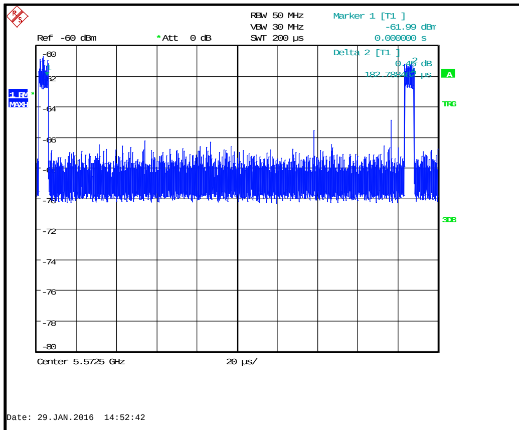
Type 2 Pulse 5µs Width 182µs PRF
