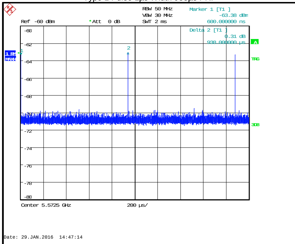
Type 1 Pulse 1 \mu s Width 938 \mu s PRF
