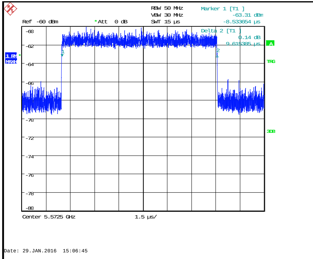
Type 3 Pulse 9.6μs Width 262μs PRF
