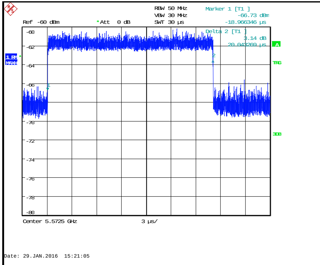
Type 4 Pulse 20µs Width 267µs PRF
